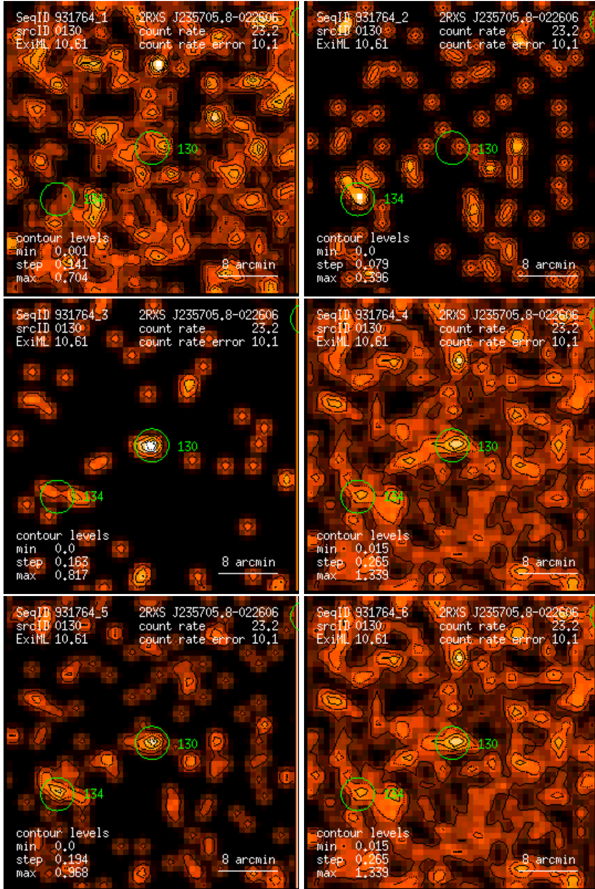
Figure 130: RASS 931764: detection 0130: band rate images, Gaussian filter: (1) PSPC channels 11 – 41, (2) 52 – 90, (3) 91 – 201, (4) 11 – 235, (5) 52 – 201, (6) 11 – 201. Broad band rates in counts/ks. Band rate contour levels in counts/ks/arcmin 2 .
