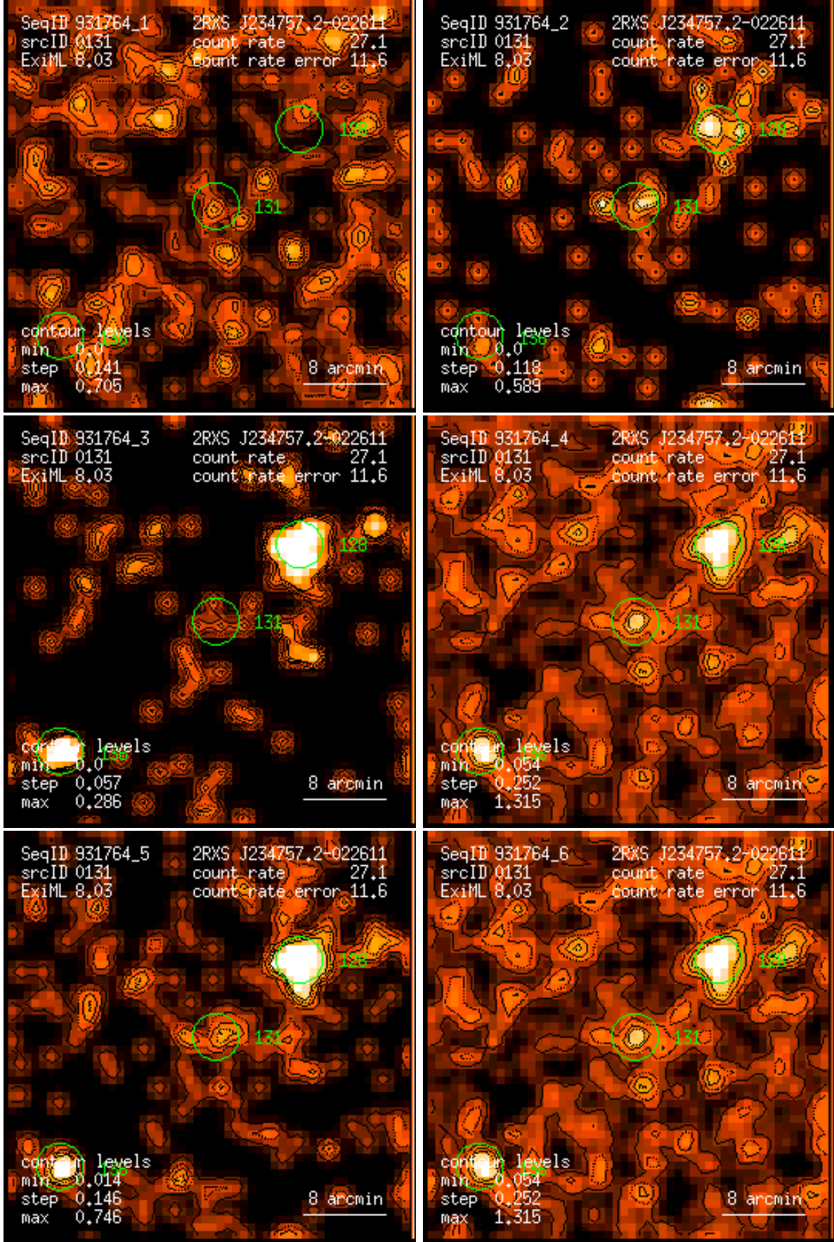
Figure 131: RASS 931764: detection 0131: band rate images, Gaussian filter: (1) PSPC channels 11 – 41, (2) 52 – 90, (3) 91 – 201, (4) 11 – 235, (5) 52 – 201, (6) 11 – 201. Broad band rates in counts/ks. Band rate contour levels in counts/ks/arcmin 2 .
