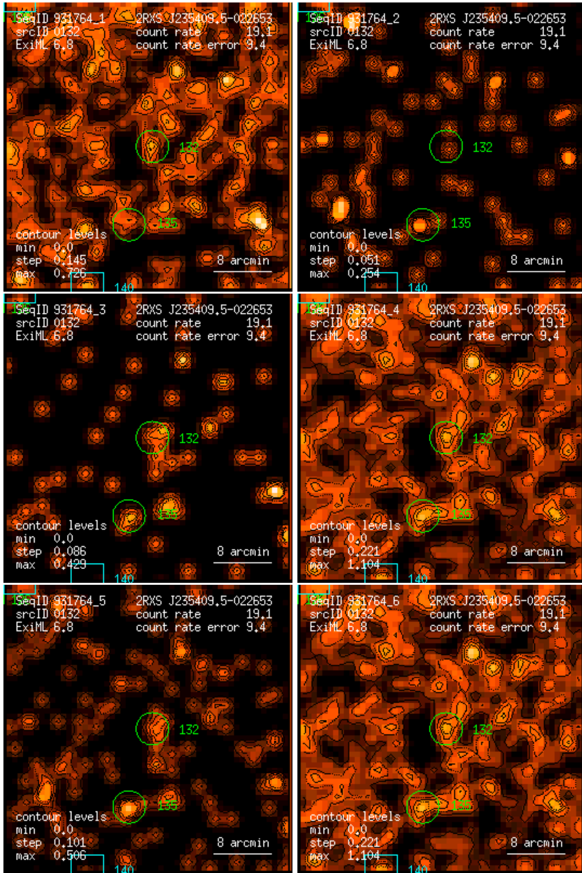
Figure 132: RASS 931764: detection 0132: band rate images, Gaussian filter: (1) PSPC channels 11 – 41, (2) 52 – 90, (3) 91 – 201, (4) 11 – 235, (5) 52 – 201, (6) 11 – 201. Broad band rates in counts/ks. Band rate contour levels in counts/ks/arcmin 2 .
