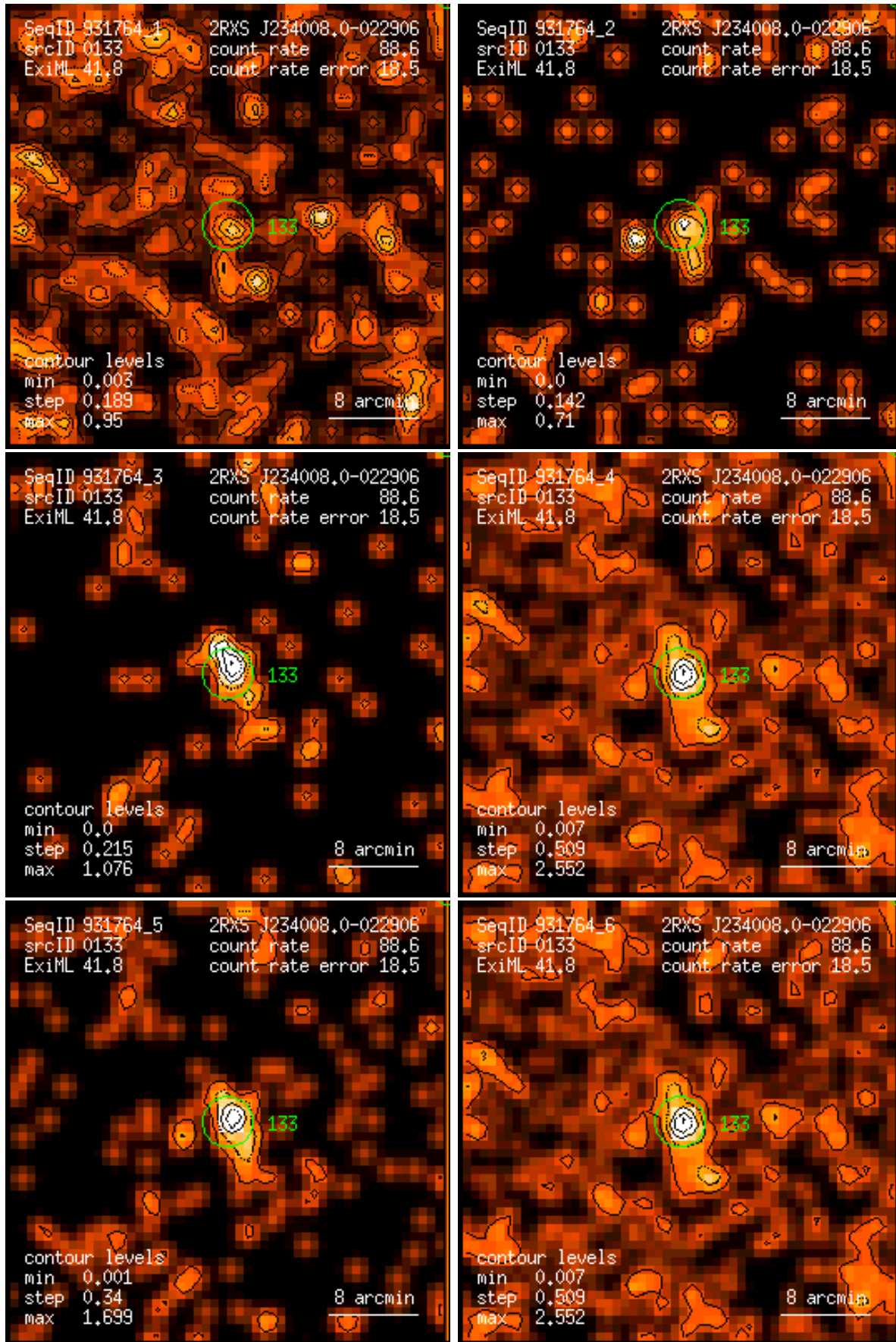
Figure 133: RASS 931764: detection 0133: band rate images, Gaussian filter: (1) PSPC channels 11 – 41, (2) 52 – 90, (3) 91 – 201, (4) 11 – 235, (5) 52 – 201, (6) 11 – 201. Broad band rates in counts/ks. Band rate contour levels in counts/ks/arcmin 2 .
