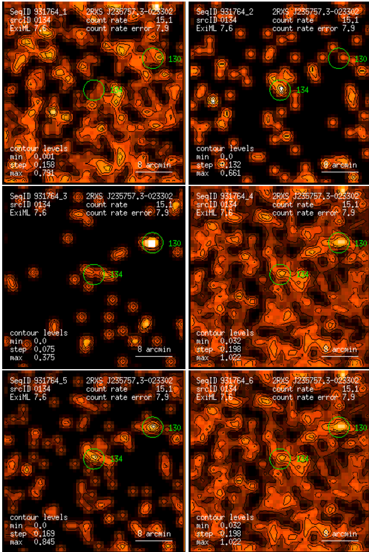
Figure 134: RASS 931764: detection 0134: band rate images, Gaussian filter: (1) PSPC channels 11 – 41, (2) 52 – 90, (3) 91 – 201, (4) 11 – 235, (5) 52 – 201, (6) 11 – 201. Broad band rates in counts/ks. Band rate contour levels in counts/ks/arcmin 2 .
