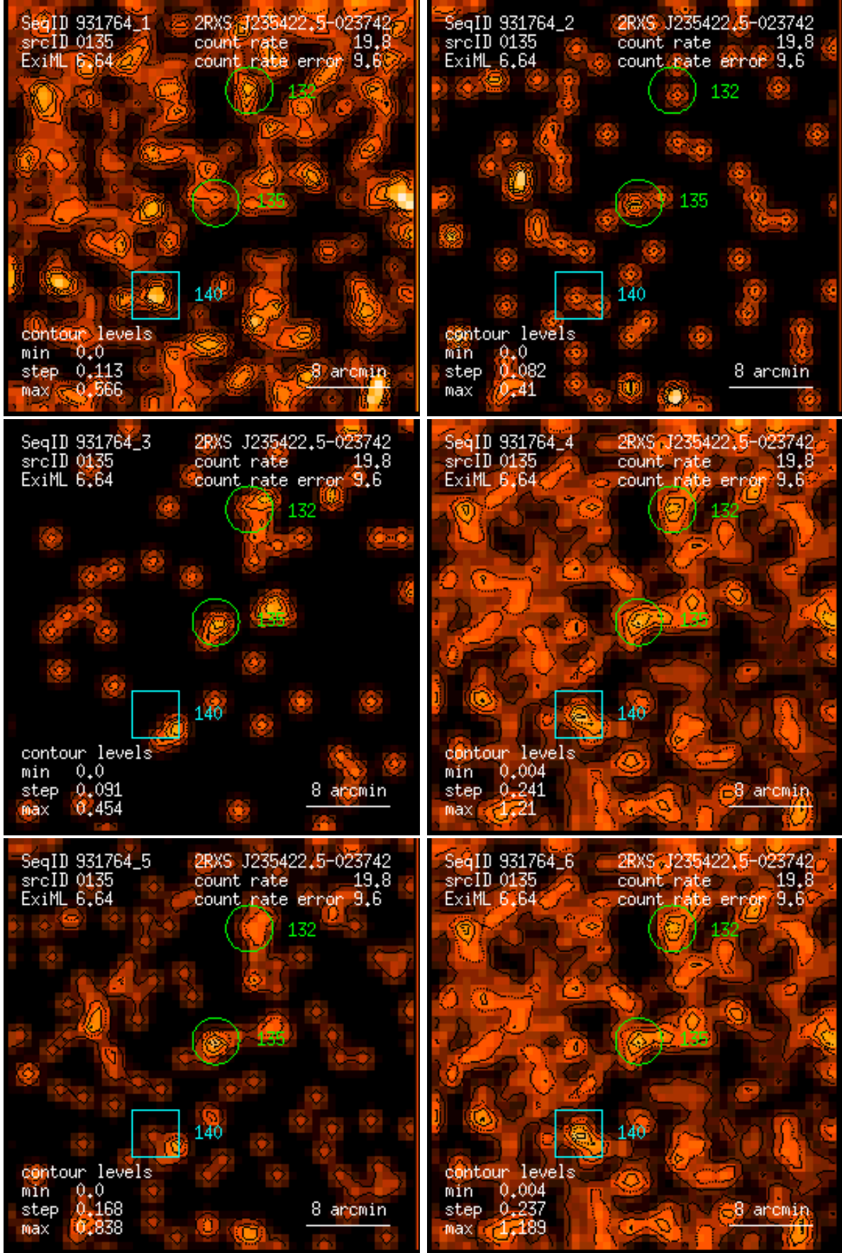
Figure 135: RASS 931764: detection 0135: band rate images, Gaussian filter: (1) PSPC channels 11 – 41, (2) 52 – 90, (3) 91 – 201, (4) 11 – 235, (5) 52 – 201, (6) 11 – 201. Broad band rates in counts/ks. Band rate contour levels in counts/ks/arcmin 2 .
