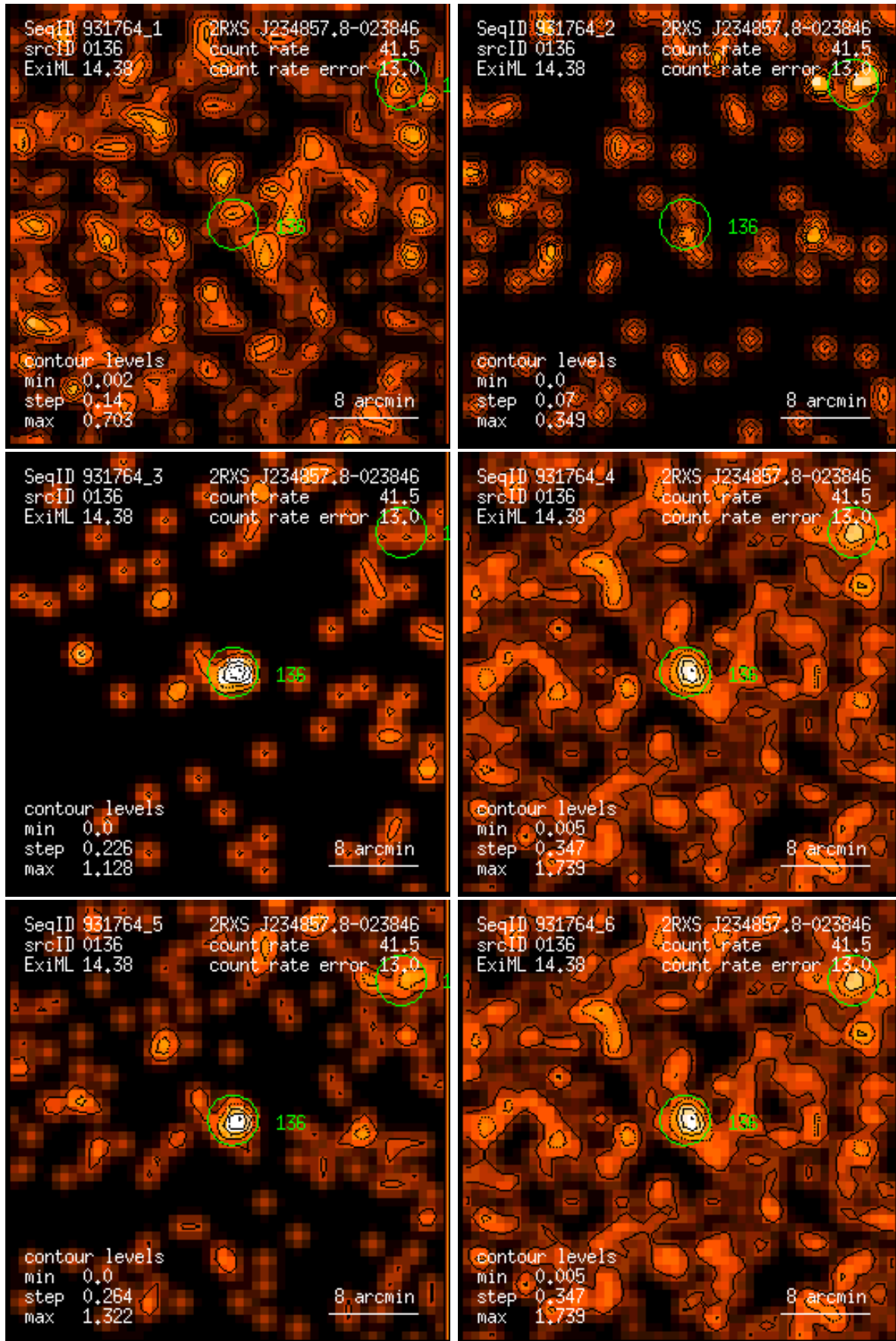
Figure 136: RASS 931764: detection 0136: band rate images, Gaussian filter: (1) PSPC channels 11 – 41, (2) 52 – 90, (3) 91 – 201, (4) 11 – 235, (5) 52 – 201, (6) 11 – 201. Broad band rates in counts/ks. Band rate contour levels in counts/ks/arcmin 2 .
