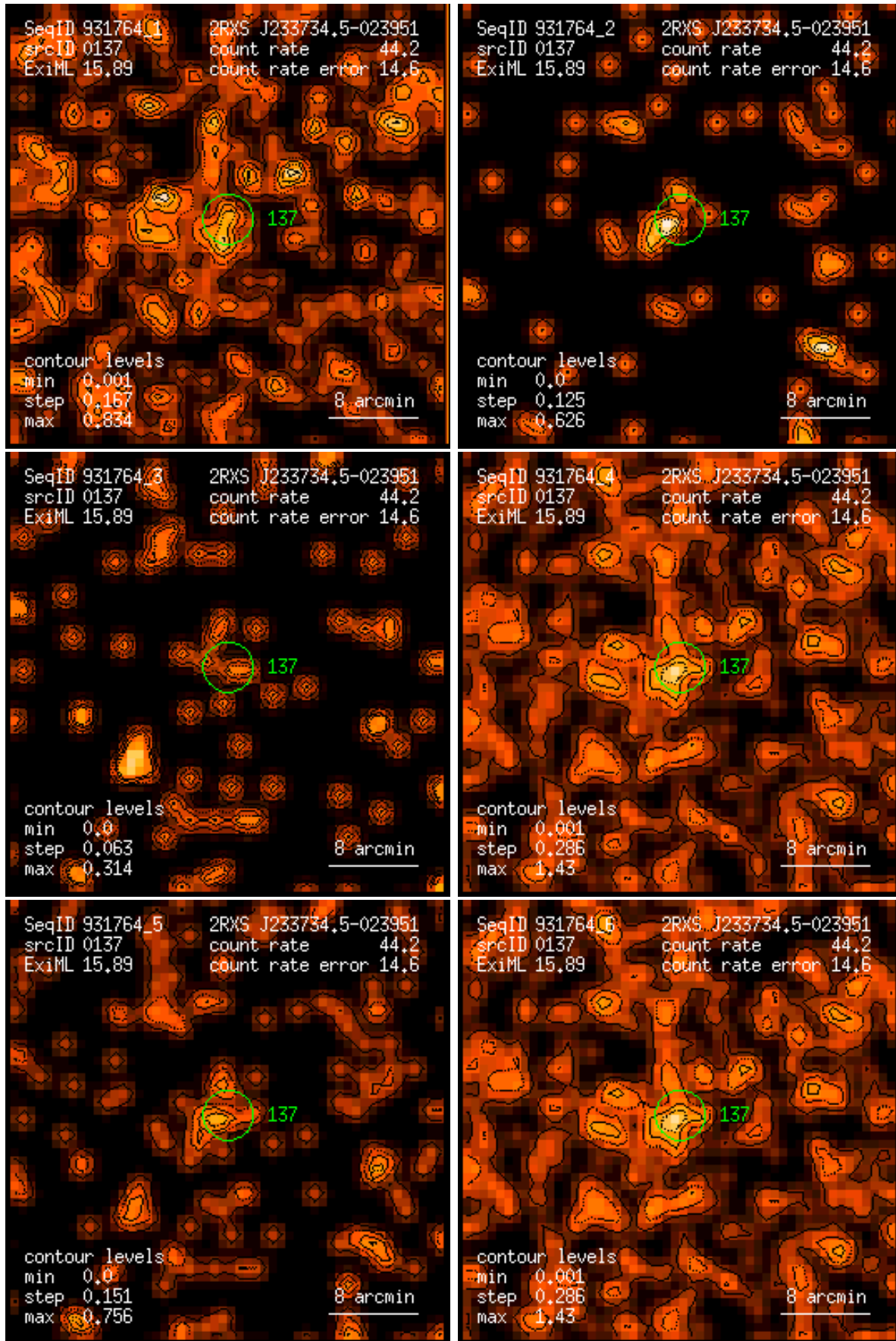
Figure 137: RASS 931764: detection 0137: band rate images, Gaussian filter: (1) PSPC channels 11 – 41, (2) 52 – 90, (3) 91 – 201, (4) 11 – 235, (5) 52 – 201, (6) 11 – 201. Broad band rates in counts/ks. Band rate contour levels in counts/ks/arcmin 2 .
