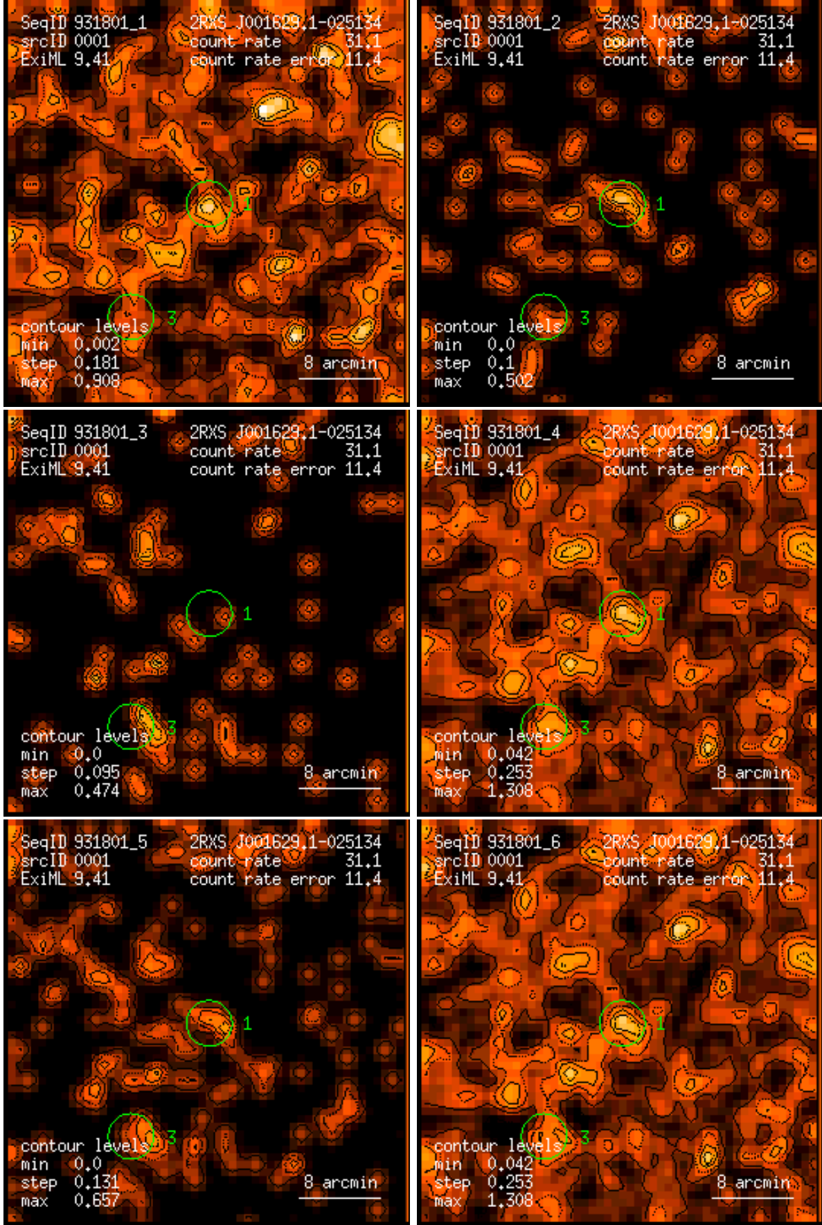
Figure 1: RASS 931801: detection 0001: band rate images, Gaussian filter: (1) PSPC channels 11 – 41, (2) 52 – 90, (3) 91 – 201, (4) 11 – 235, (5) 52 – 201, (6) 11 – 201. Broad band rates in counts/ks. Band rate contour levels in counts/ks/arcmin 2 .
