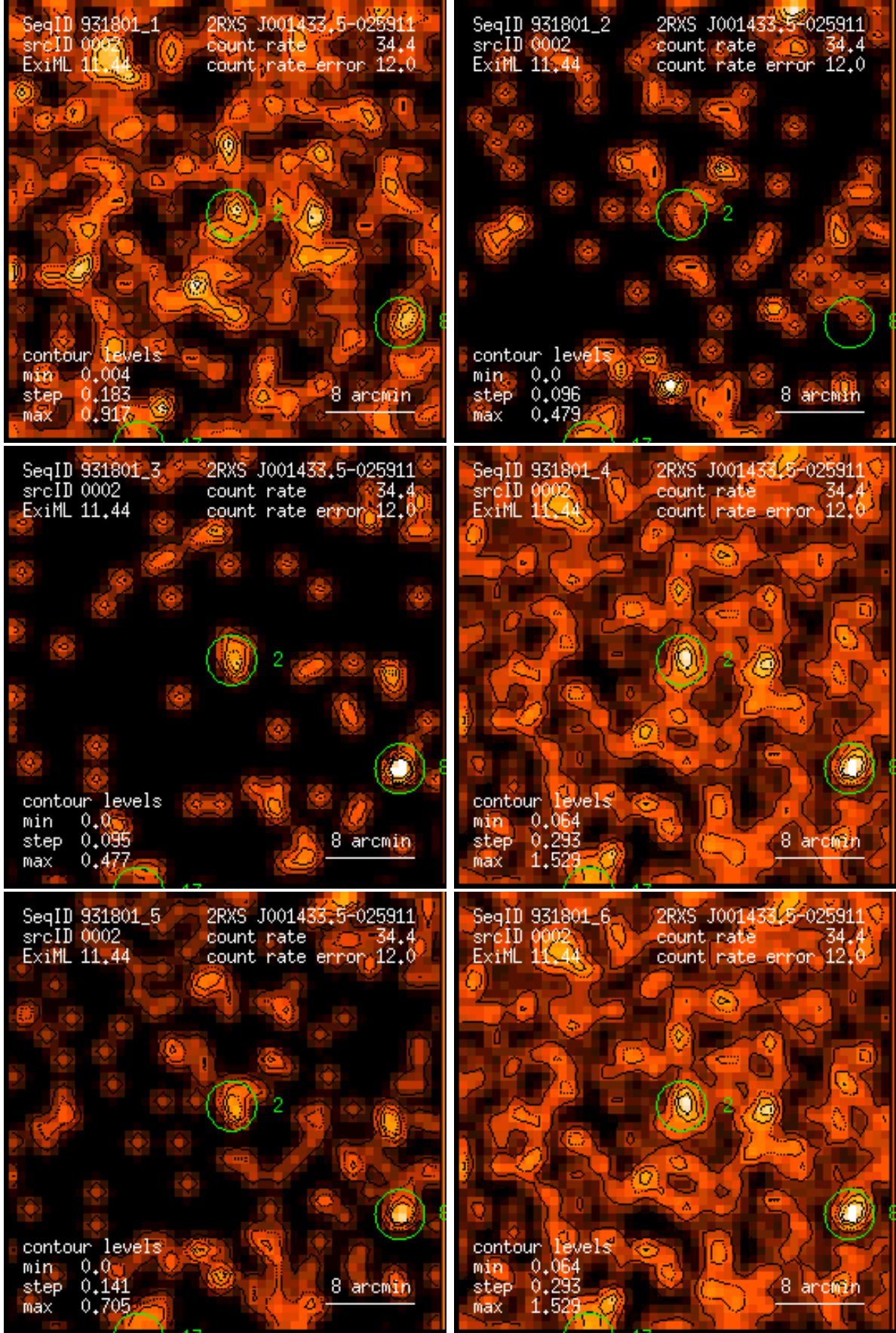
Figure 2: RASS 931801: detection 0002: band rate images, Gaussian filter: (1) PSPC channels 11 – 41, (2) 52 – 90, (3) 91 – 201, (4) 11 – 235, (5) 52 – 201, (6) 11 – 201. Broad band rates in counts/ks. Band rate contour levels in counts/ks/arcmin 2 .
