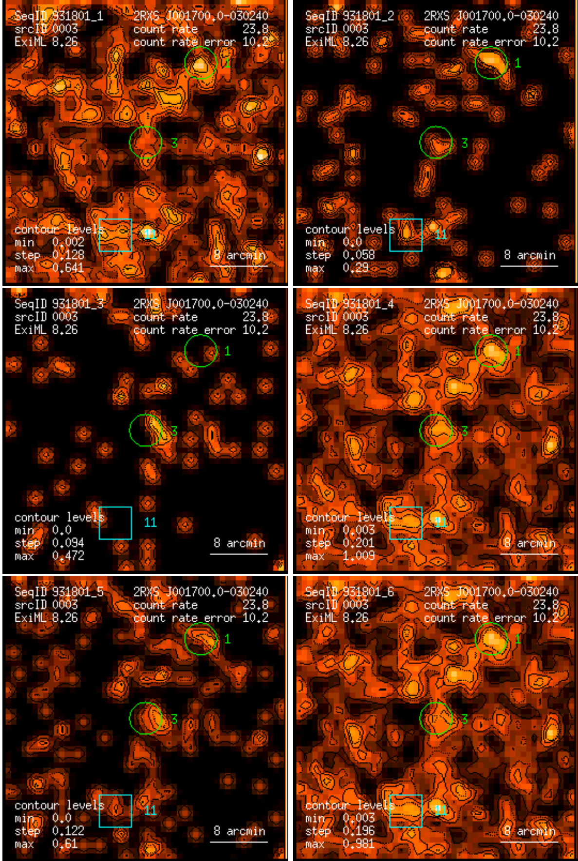
Figure 3: RASS 931801: detection 0003: band rate images, Gaussian filter: (1) PSPC channels 11 – 41, (2) 52 – 90, (3) 91 – 201, (4) 11 – 235, (5) 52 – 201, (6) 11 – 201. Broad band rates in counts/ks. Band rate contour levels in counts/ks/arcmin 2 .
