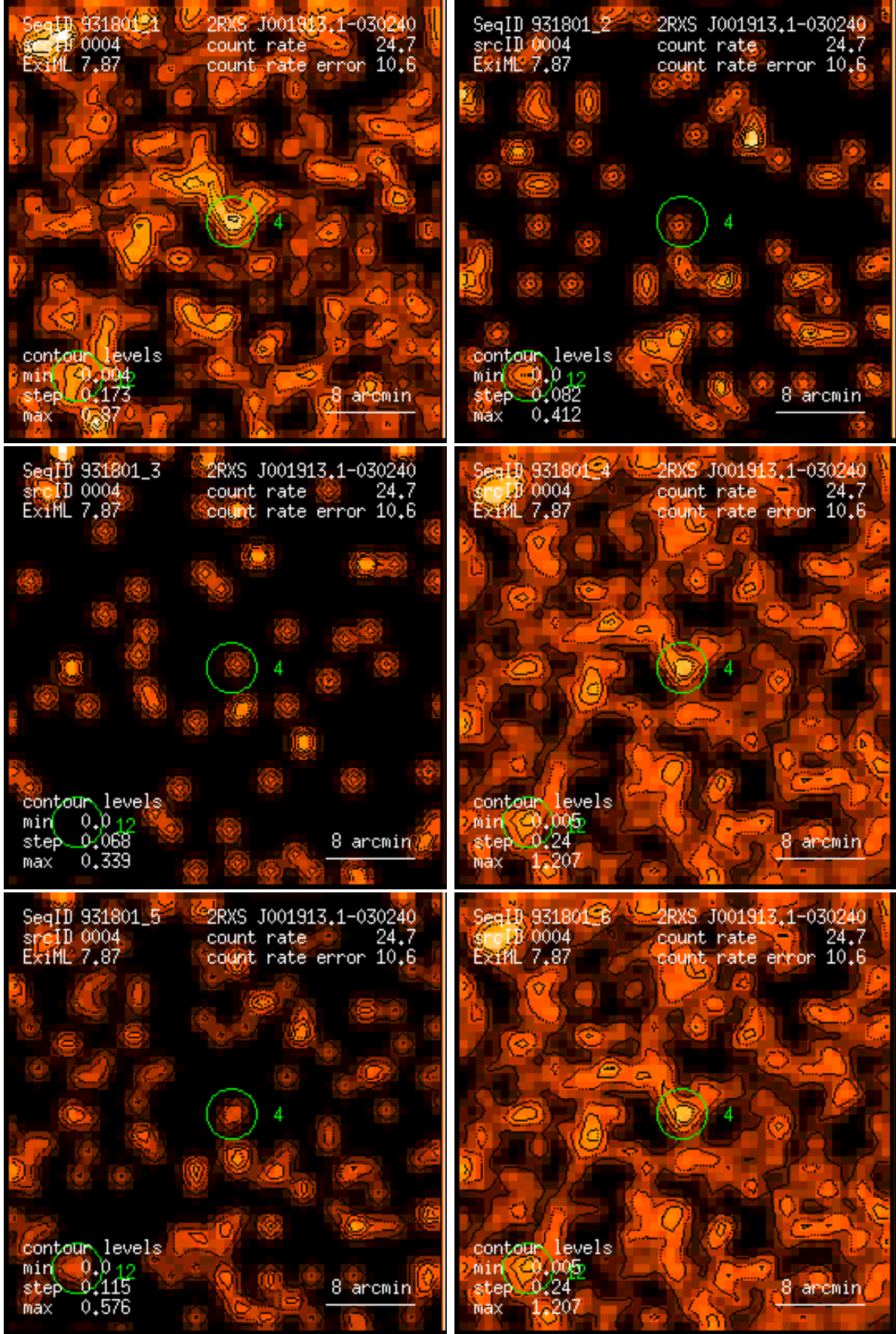
Figure 4: RASS 931801: detection 0004: band rate images, Gaussian filter: (1) PSPC channels 11 – 41, (2) 52 – 90, (3) 91 – 201, (4) 11 – 235, (5) 52 – 201, (6) 11 – 201. Broad band rates in counts/ks. Band rate contour levels in counts/ks/arcmin 2 .
