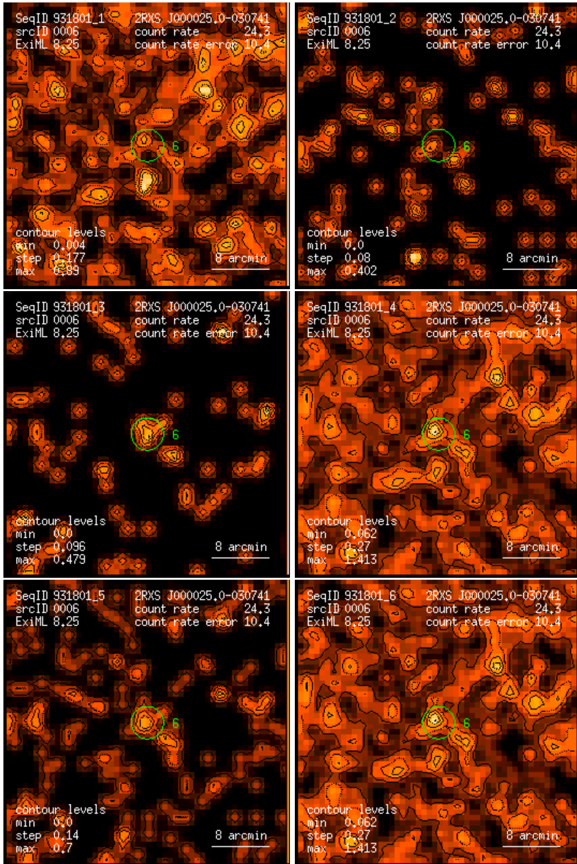
Figure 6: RASS 931801: detection 0006: band rate images, Gaussian filter: (1) PSPC channels 11 – 41, (2) 52 – 90, (3) 91 – 201, (4) 11 – 235, (5) 52 – 201, (6) 11 – 201. Broad band rates in counts/ks. Band rate contour levels in counts/ks/arcmin 2 .
