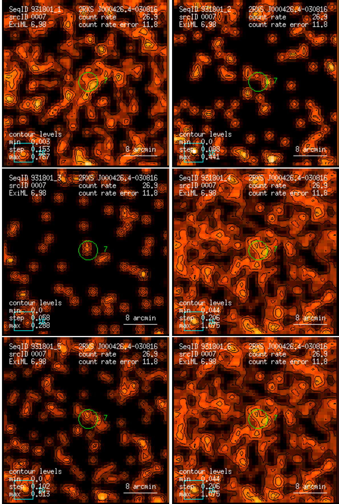
Figure 7: RASS 931801: detection 0007: band rate images, Gaussian filter: (1) PSPC channels 11 – 41, (2) 52 – 90, (3) 91 – 201, (4) 11 – 235, (5) 52 – 201, (6) 11 – 201. Broad band rates in counts/ks. Band rate contour levels in counts/ks/arcmin 2 .
