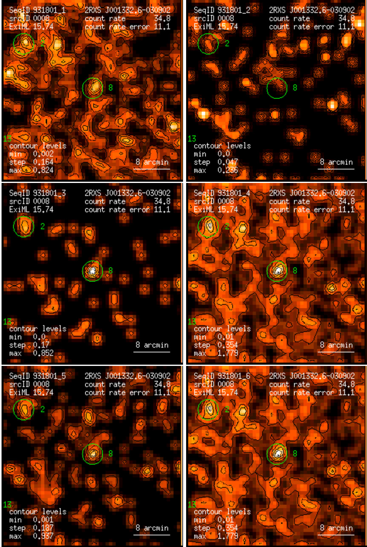
Figure 8: RASS 931801: detection 0008: band rate images, Gaussian filter: (1) PSPC channels 11 – 41, (2) 52 – 90, (3) 91 – 201, (4) 11 – 235, (5) 52 – 201, (6) 11 – 201. Broad band rates in counts/ks. Band rate contour levels in counts/ks/arcmin 2 .
