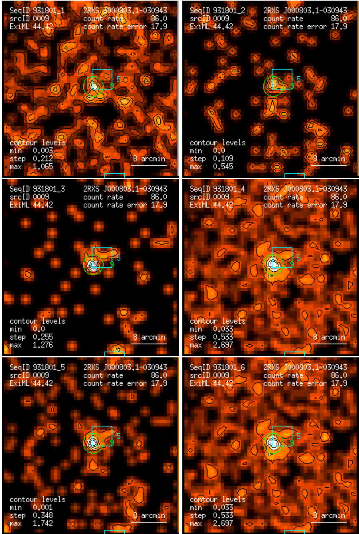
Figure 9: RASS 931801: detection 0009: band rate images, Gaussian filter: (1) PSPC channels 11 – 41, (2) 52 – 90, (3) 91 – 201, (4) 11 – 235, (5) 52 – 201, (6) 11 – 201. Broad band rates in counts/ks. Band rate contour levels in counts/ks/arcmin 2 .
