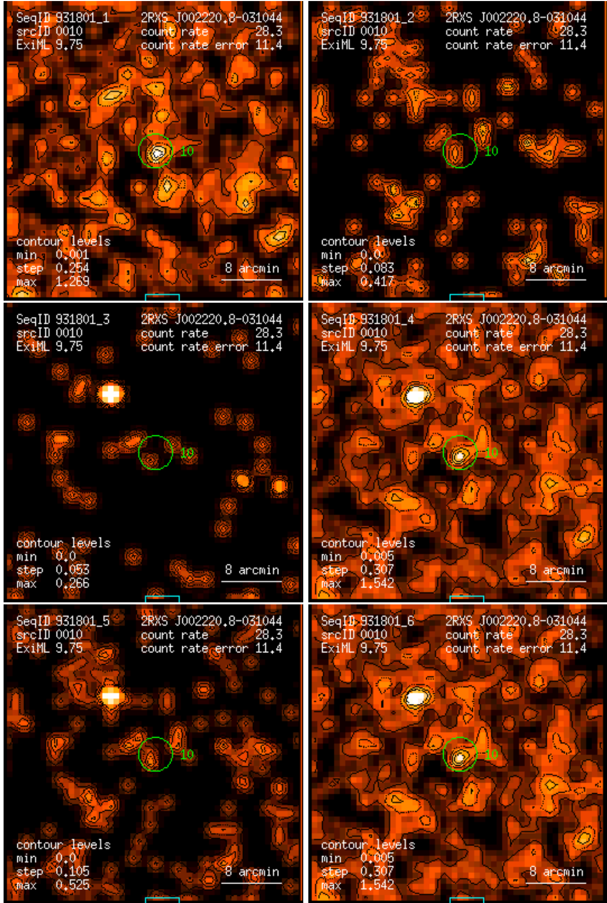
Figure 10: RASS 931801: detection 0010: band rate images, Gaussian filter: (1) PSPC channels 11 – 41, (2) 52 – 90, (3) 91 – 201, (4) 11 – 235, (5) 52 – 201, (6) 11 – 201. Broad band rates in counts/ks. Band rate contour levels in counts/ks/arcmin 2 .
