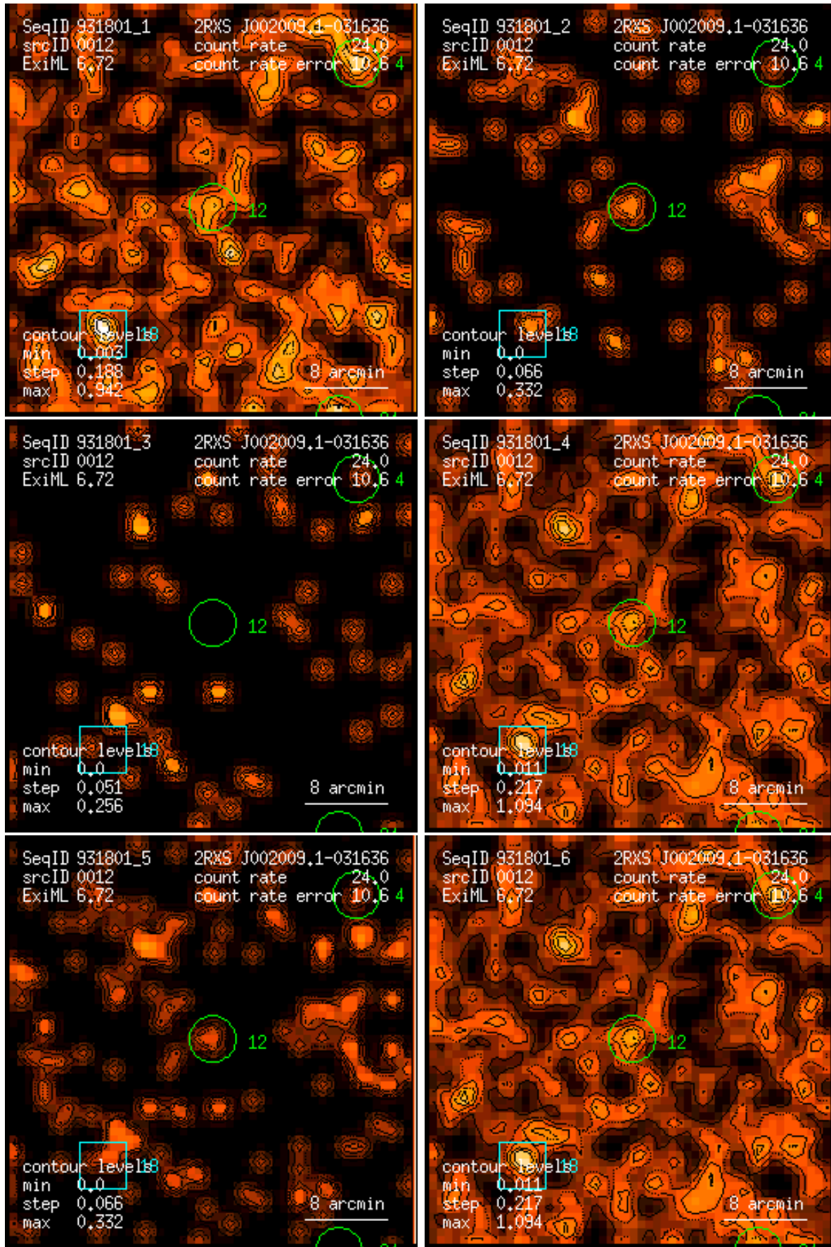
Figure 12: RASS 931801: detection 0012: band rate images, Gaussian filter: (1) PSPC channels 11 – 41, (2) 52 – 90, (3) 91 – 201, (4) 11 – 235, (5) 52 – 201, (6) 11 – 201. Broad band rates in counts/ks. Band rate contour levels in counts/ks/arcmin 2 .
