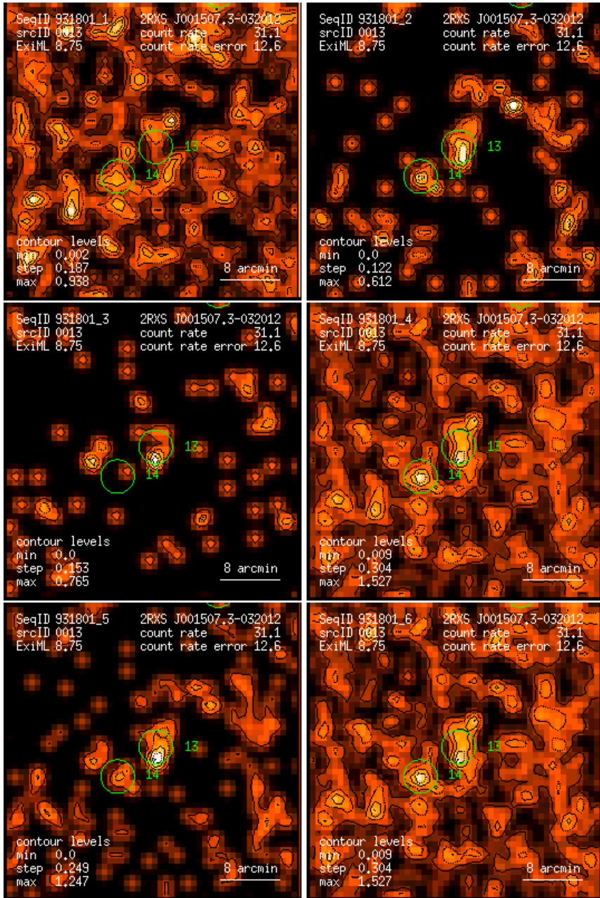
Figure 13: RASS 931801: detection 0013: band rate images, Gaussian filter: (1) PSPC channels 11 – 41, (2) 52 – 90, (3) 91 – 201, (4) 11 – 235, (5) 52 – 201, (6) 11 – 201. Broad band rates in counts/ks. Band rate contour levels in counts/ks/arcmin 2 .
