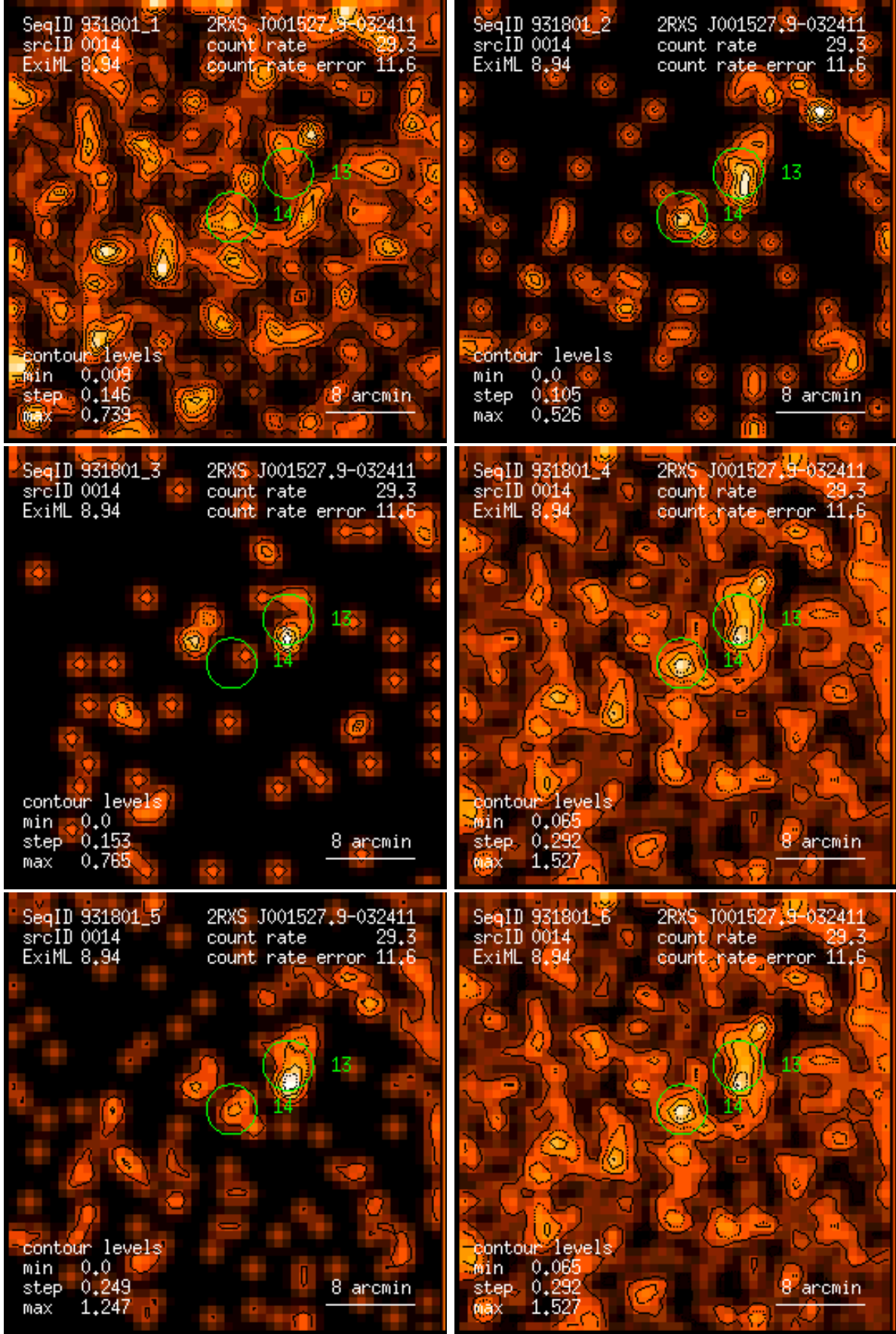
Figure 14: RASS 931801: detection 0014: band rate images, Gaussian filter: (1) PSPC channels 11 – 41, (2) 52 – 90, (3) 91 – 201, (4) 11 – 235, (5) 52 – 201, (6) 11 – 201. Broad band rates in counts/ks. Band rate contour levels in counts/ks/arcmin 2 .
