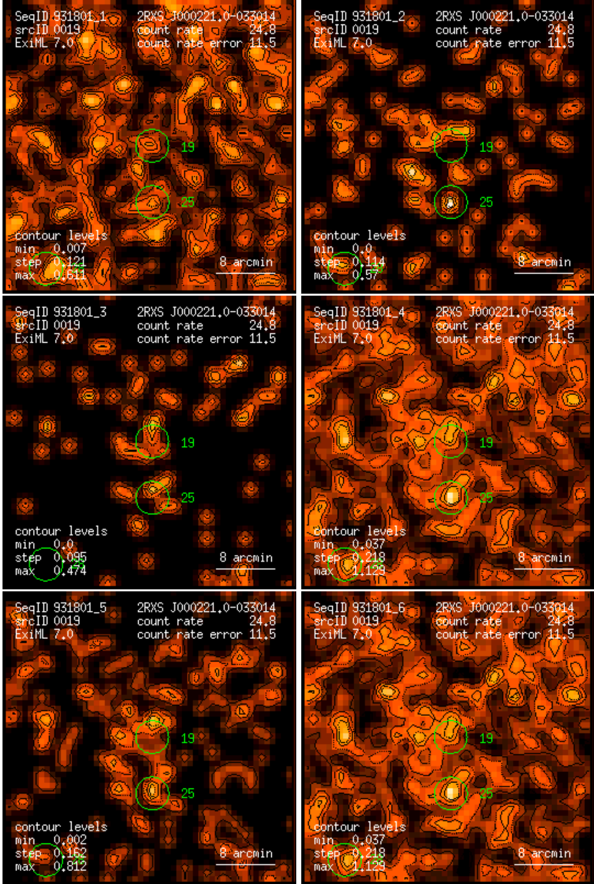
Figure 19: RASS 931801: detection 0019: band rate images, Gaussian filter: (1) PSPC channels 11 – 41, (2) 52 – 90, (3) 91 – 201, (4) 11 – 235, (5) 52 – 201, (6) 11 – 201. Broad band rates in counts/ks. Band rate contour levels in counts/ks/arcmin 2 .
