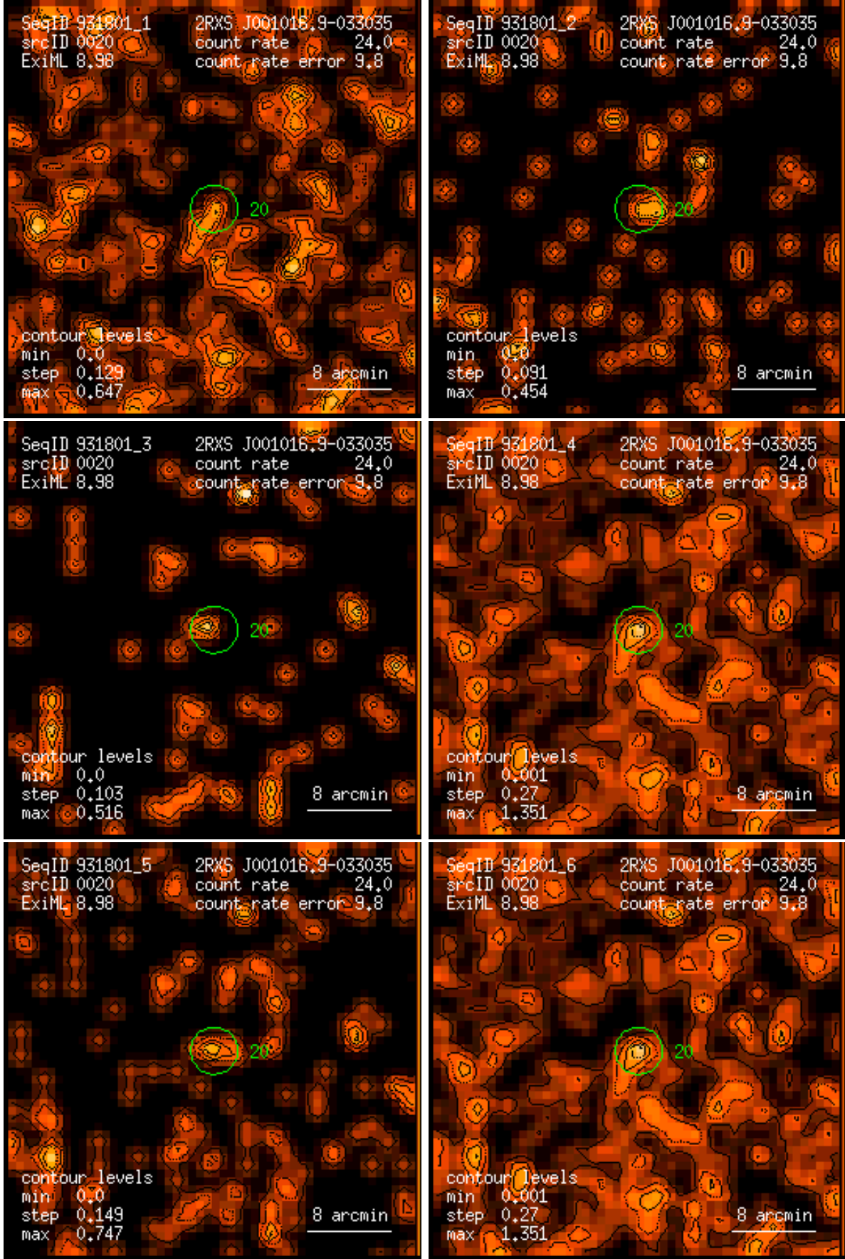
Figure 20: RASS 931801: detection 0020: band rate images, Gaussian filter: (1) PSPC channels 11 – 41, (2) 52 – 90, (3) 91 – 201, (4) 11 – 235, (5) 52 – 201, (6) 11 – 201. Broad band rates in counts/ks. Band rate contour levels in counts/ks/arcmin 2 .
