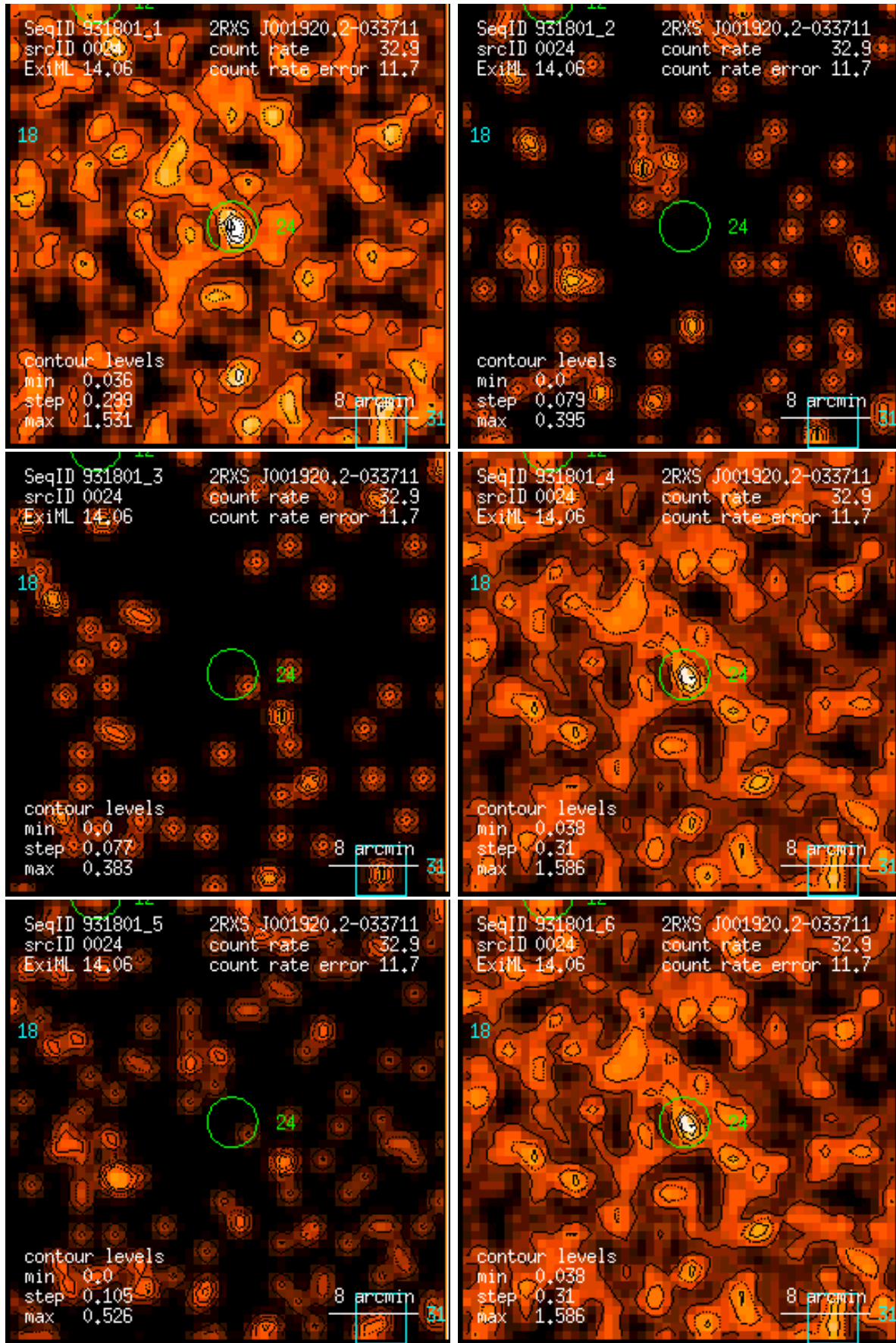
Figure 24: RASS 931801: detection 0024: band rate images, Gaussian filter: (1) PSPC channels 11 – 41, (2) 52 – 90, (3) 91 – 201, (4) 11 – 235, (5) 52 – 201, (6) 11 – 201. Broad band rates in counts/ks. Band rate contour levels in counts/ks/arcmin 2 .
