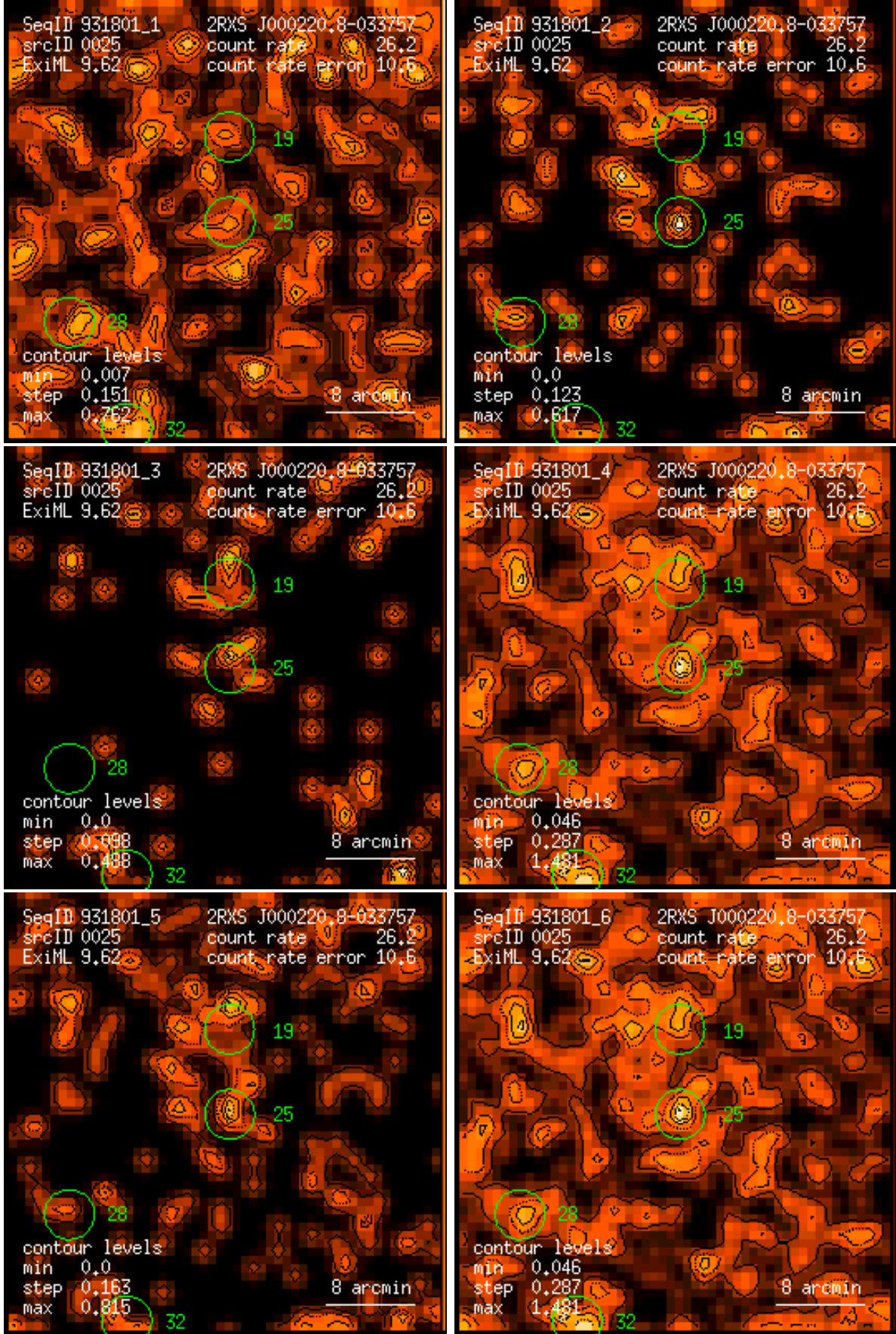
Figure 25: RASS 931801: detection 0025: band rate images, Gaussian filter: (1) PSPC channels 11 – 41, (2) 52 – 90, (3) 91 – 201, (4) 11 – 235, (5) 52 – 201, (6) 11 – 201. Broad band rates in counts/ks. Band rate contour levels in counts/ks/arcmin 2 .
