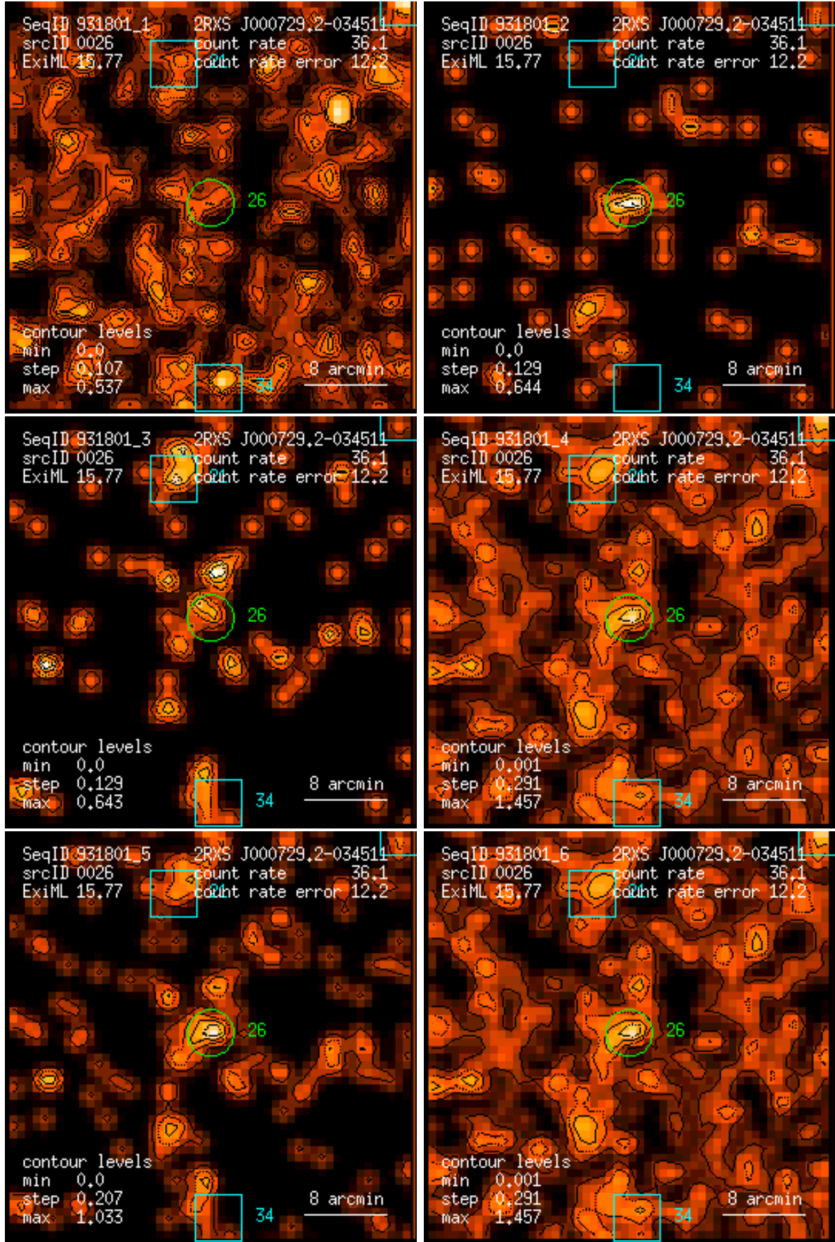
Figure 26: RASS 931801: detection 0026: band rate images, Gaussian filter: (1) PSPC channels 11 – 41, (2) 52 – 90, (3) 91 – 201, (4) 11 – 235, (5) 52 – 201, (6) 11 – 201. Broad band rates in counts/ks. Band rate contour levels in counts/ks/arcmin 2 .
