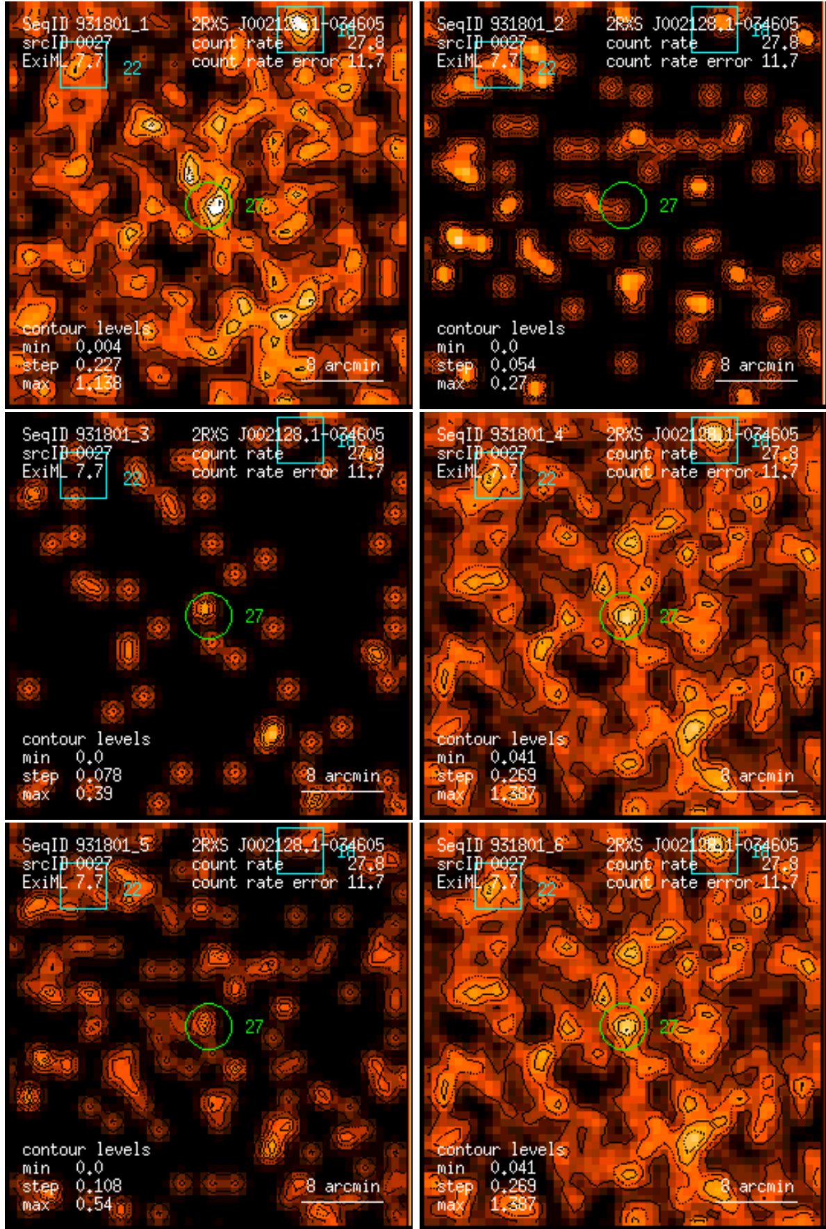
Figure 27: RASS 931801: detection 0027: band rate images, Gaussian filter: (1) PSPC channels 11 – 41, (2) 52 – 90, (3) 91 – 201, (4) 11 – 235, (5) 52 – 201, (6) 11 – 201. Broad band rates in counts/ks. Band rate contour levels in counts/ks/arcmin 2 .
