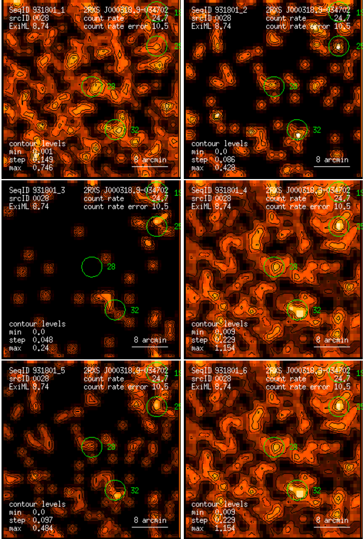
Figure 28: RASS 931801: detection 0028: band rate images, Gaussian filter: (1) PSPC channels 11 – 41, (2) 52 – 90, (3) 91 – 201, (4) 11 – 235, (5) 52 – 201, (6) 11 – 201. Broad band rates in counts/ks. Band rate contour levels in counts/ks/arcmin 2 .
