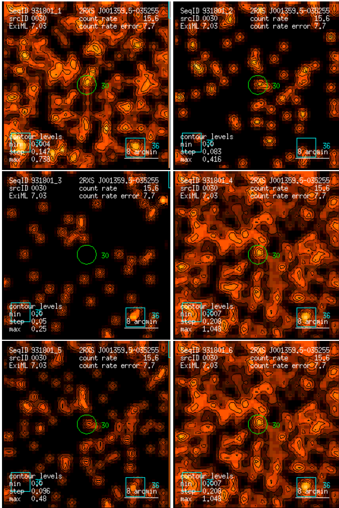
Figure 30: RASS 931801: detection 0030: band rate images, Gaussian filter: (1) PSPC channels 11 – 41, (2) 52 – 90, (3) 91 – 201, (4) 11 – 235, (5) 52 – 201, (6) 11 – 201. Broad band rates in counts/ks. Band rate contour levels in counts/ks/arcmin 2 .
