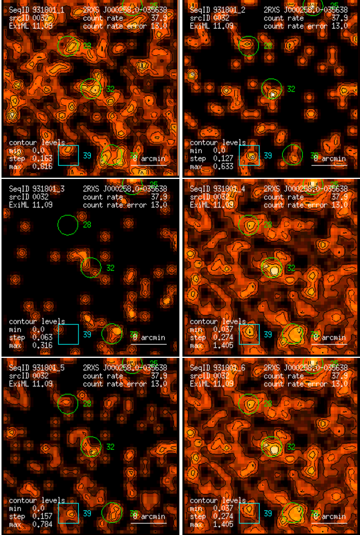
Figure 32: RASS 931801: detection 0032: band rate images, Gaussian filter: (1) PSPC channels 11 – 41, (2) 52 – 90, (3) 91 – 201, (4) 11 – 235, (5) 52 – 201, (6) 11 – 201. Broad band rates in counts/ks. Band rate contour levels in counts/ks/arcmin 2 .
