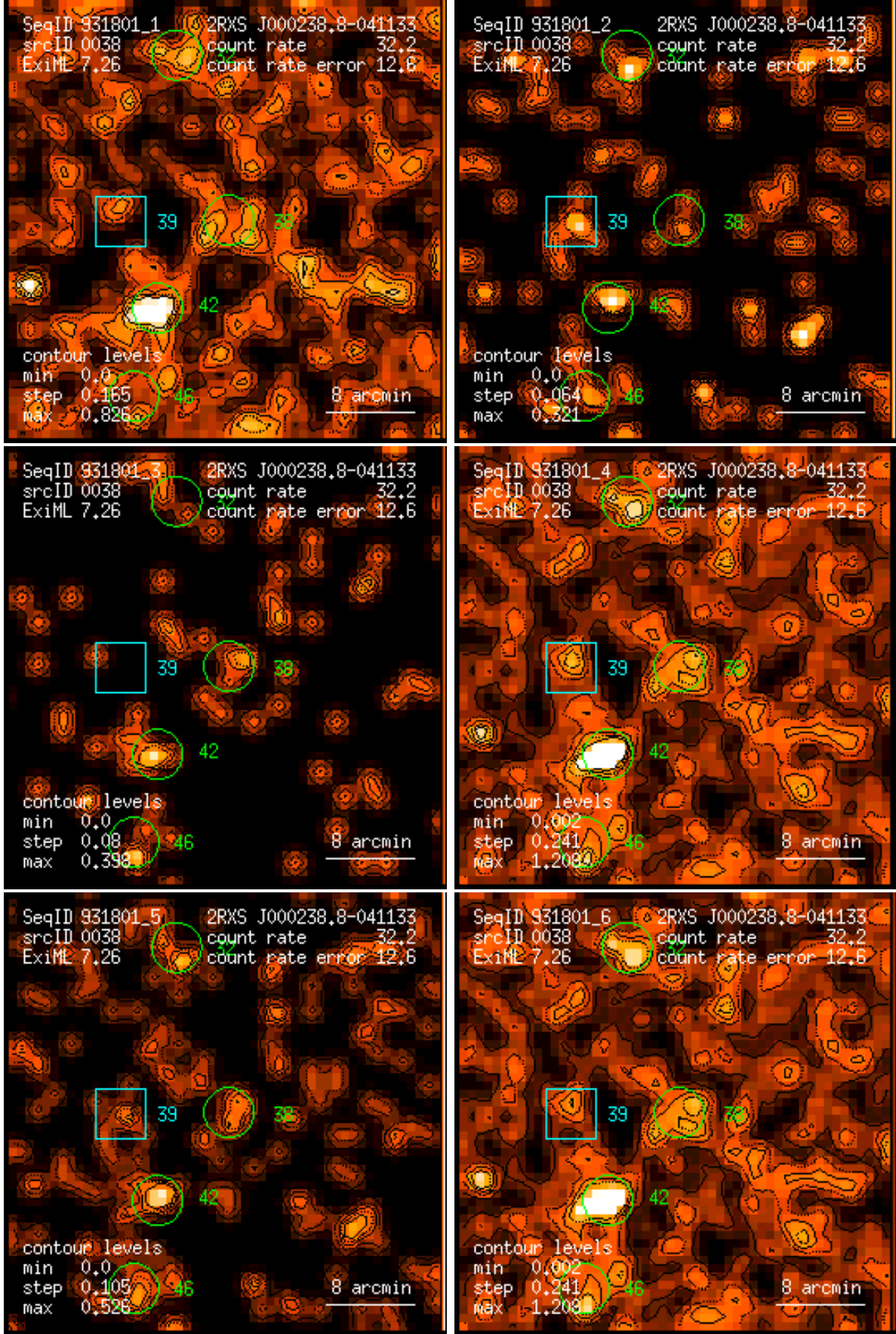
Figure 38: RASS 931801: detection 0038: band rate images, Gaussian filter: (1) PSPC channels 11 – 41, (2) 52 – 90, (3) 91 – 201, (4) 11 – 235, (5) 52 – 201, (6) 11 – 201. Broad band rates in counts/ks. Band rate contour levels in counts/ks/arcmin 2 .
