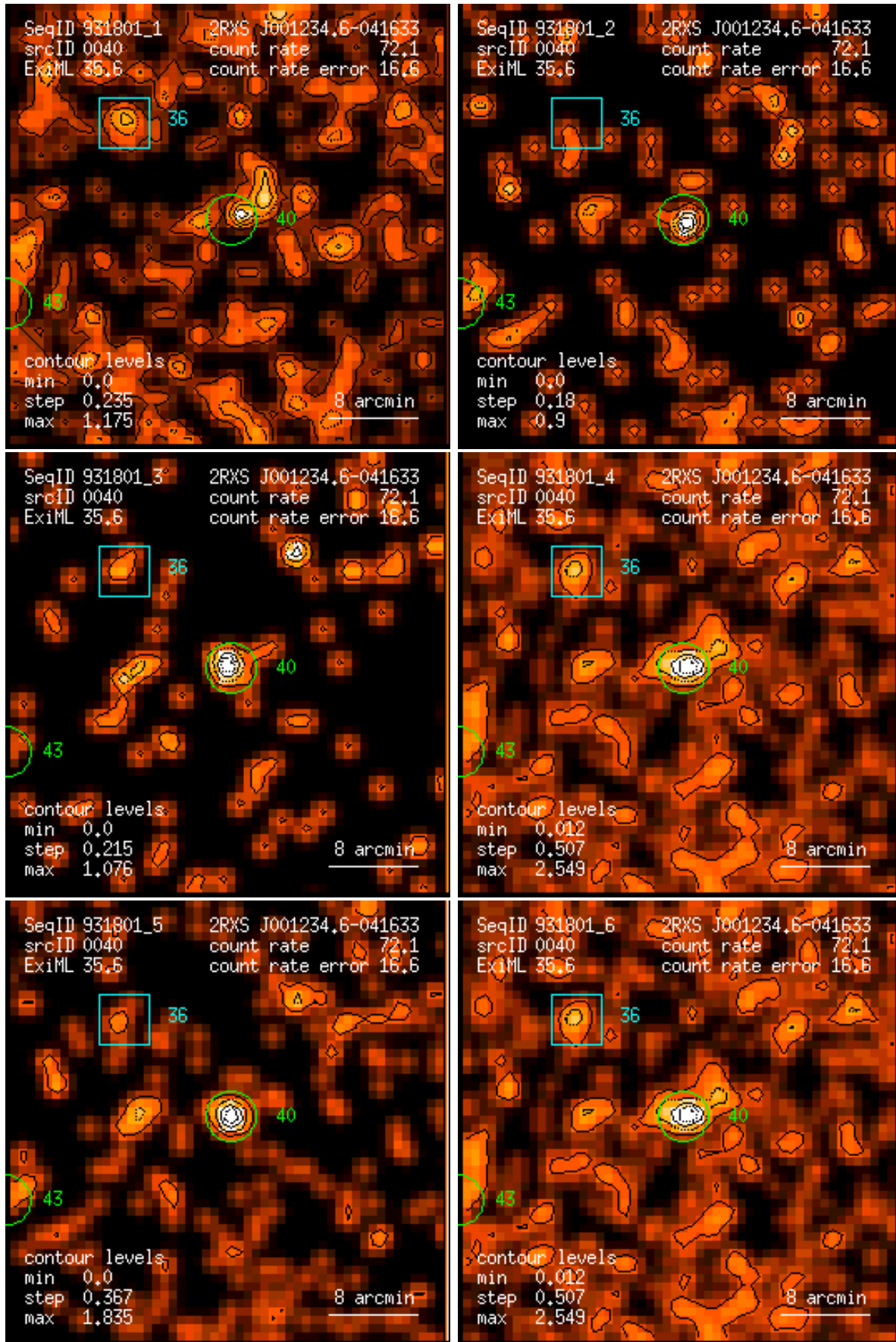
Figure 40: RASS 931801: detection 0040: band rate images, Gaussian filter: (1) PSPC channels 11 – 41, (2) 52 – 90, (3) 91 – 201, (4) 11 – 235, (5) 52 – 201, (6) 11 – 201. Broad band rates in counts/ks. Band rate contour levels in counts/ks/arcmin 2 .
