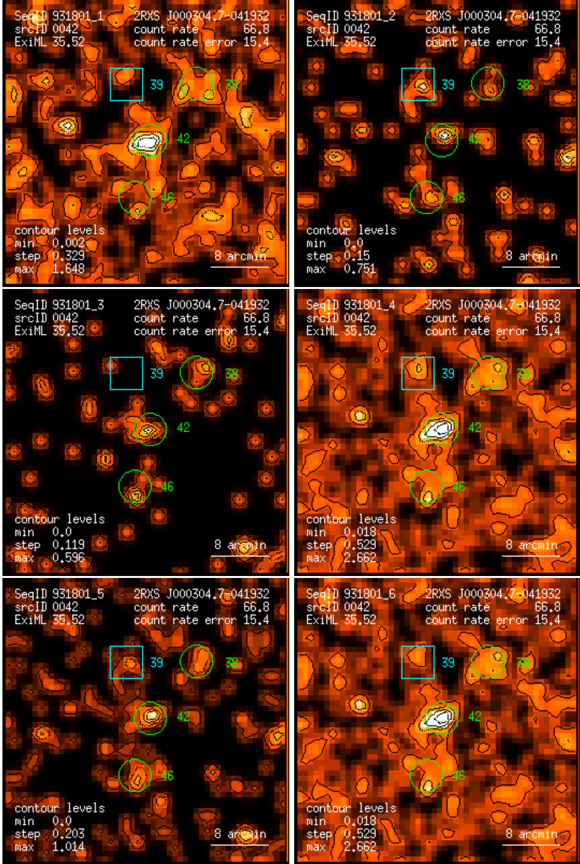
Figure 42: RASS 931801: detection 0042: band rate images, Gaussian filter: (1) PSPC channels 11 – 41, (2) 52 – 90, (3) 91 – 201, (4) 11 – 235, (5) 52 – 201, (6) 11 – 201. Broad band rates in counts/ks. Band rate contour levels in counts/ks/arcmin 2 .
