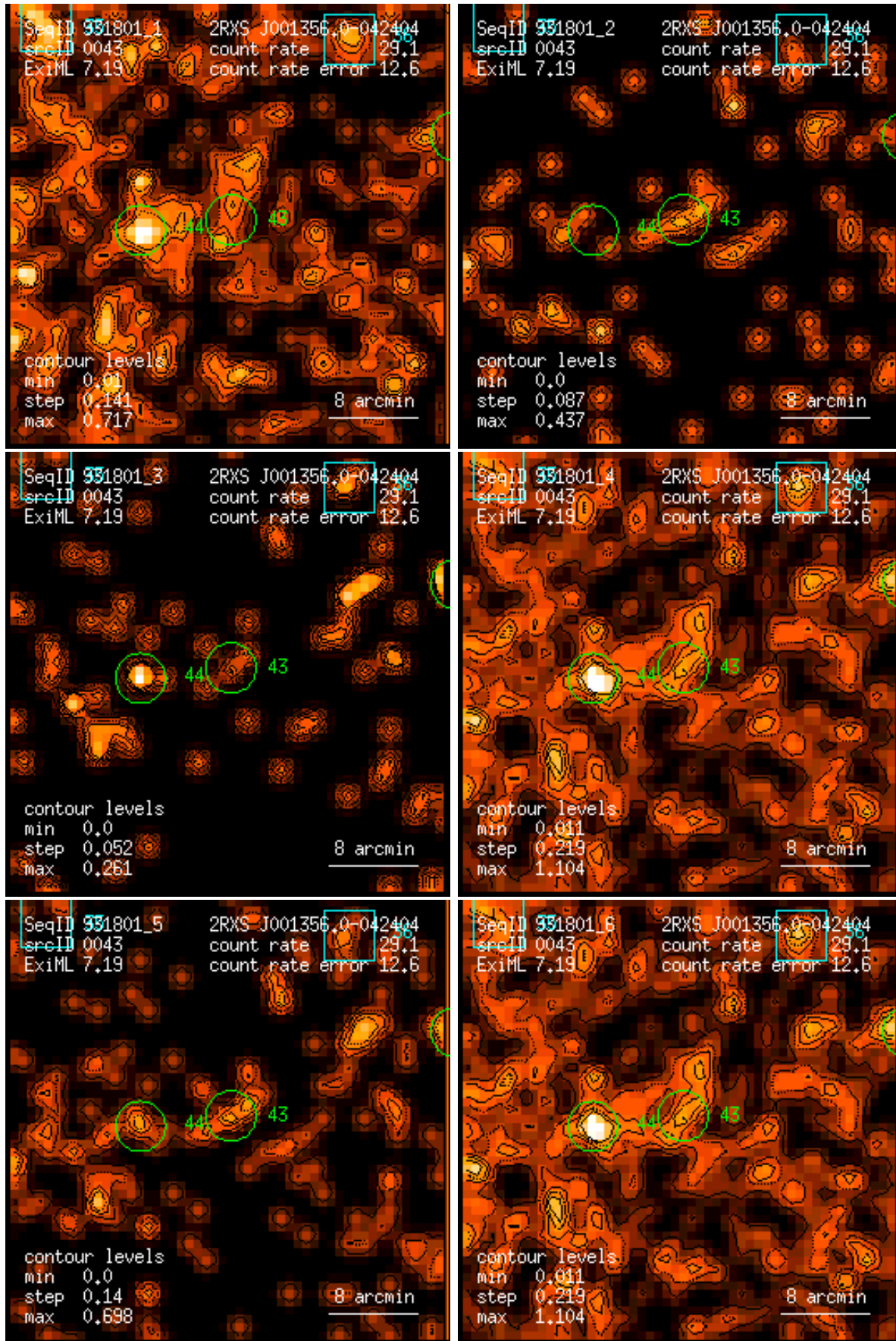
Figure 43: RASS 931801: detection 0043: band rate images, Gaussian filter: (1) PSPC channels 11 – 41, (2) 52 – 90, (3) 91 – 201, (4) 11 – 235, (5) 52 – 201, (6) 11 – 201. Broad band rates in counts/ks. Band rate contour levels in counts/ks/arcmin 2 .
