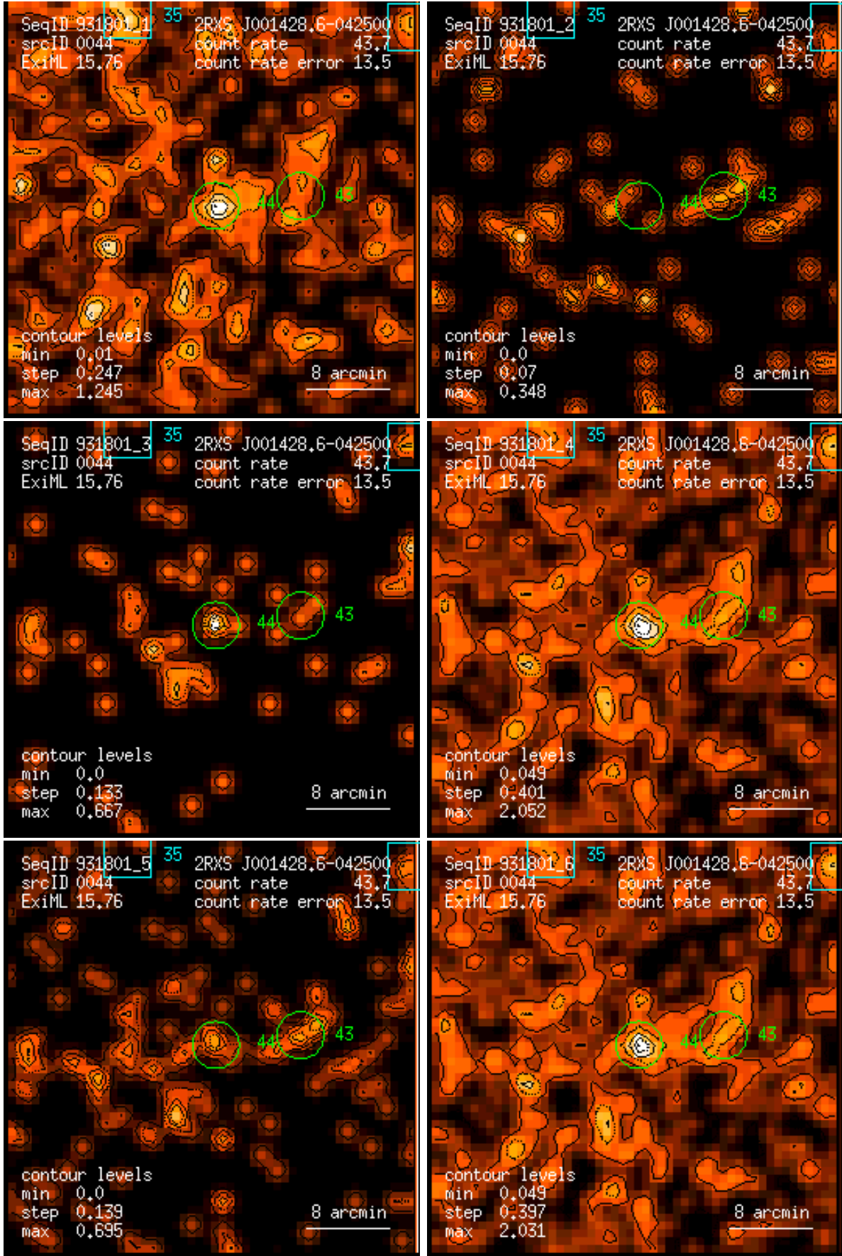
Figure 44: RASS 931801: detection 0044: band rate images, Gaussian filter: (1) PSPC channels 11 – 41, (2) 52 – 90, (3) 91 – 201, (4) 11 – 235, (5) 52 – 201, (6) 11 – 201. Broad band rates in counts/ks. Band rate contour levels in counts/ks/arcmin 2 .
