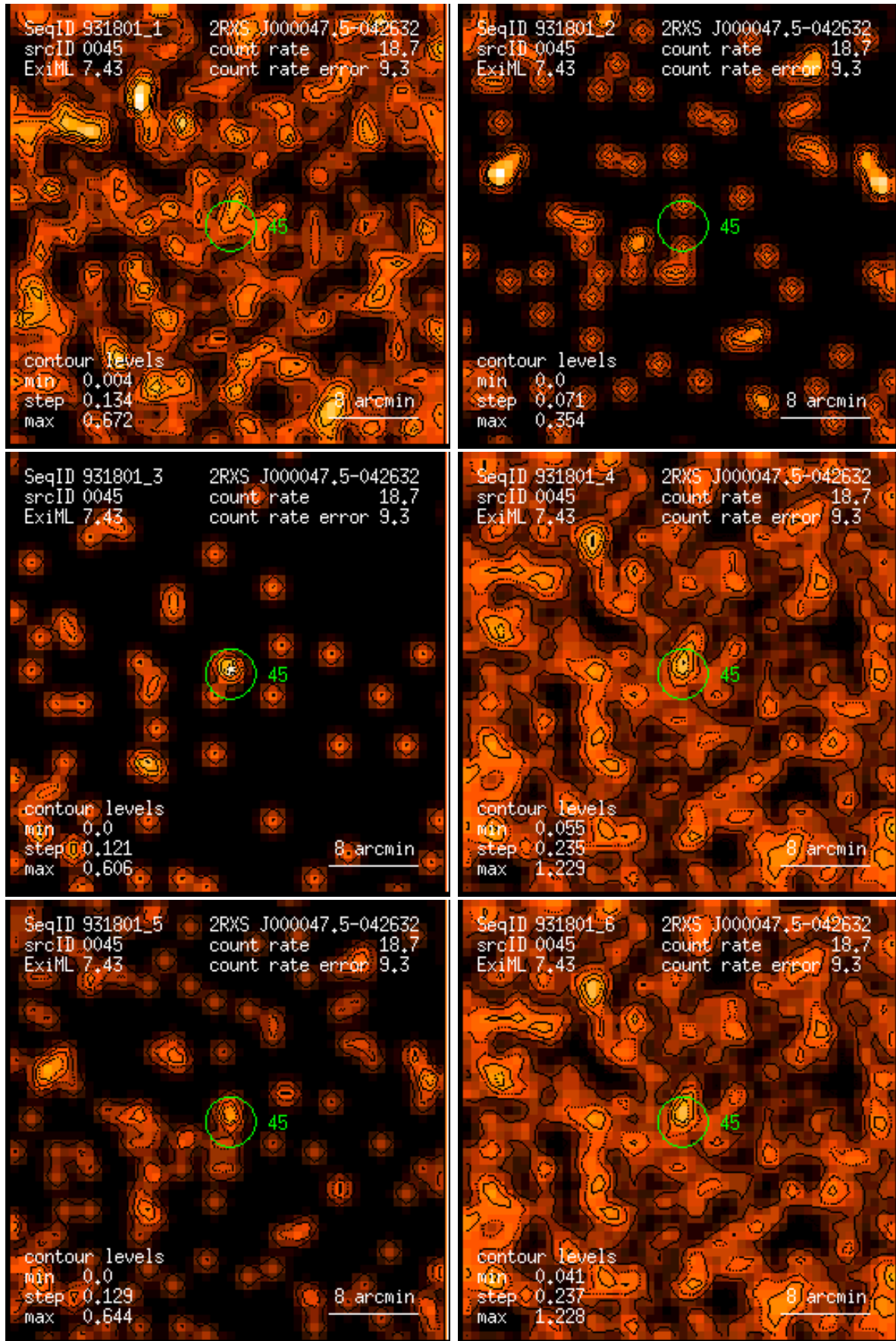
Figure 45: RASS 931801: detection 0045: band rate images, Gaussian filter: (1) PSPC channels 11 – 41, (2) 52 – 90, (3) 91 – 201, (4) 11 – 235, (5) 52 – 201, (6) 11 – 201. Broad band rates in counts/ks. Band rate contour levels in counts/ks/arcmin 2 .
