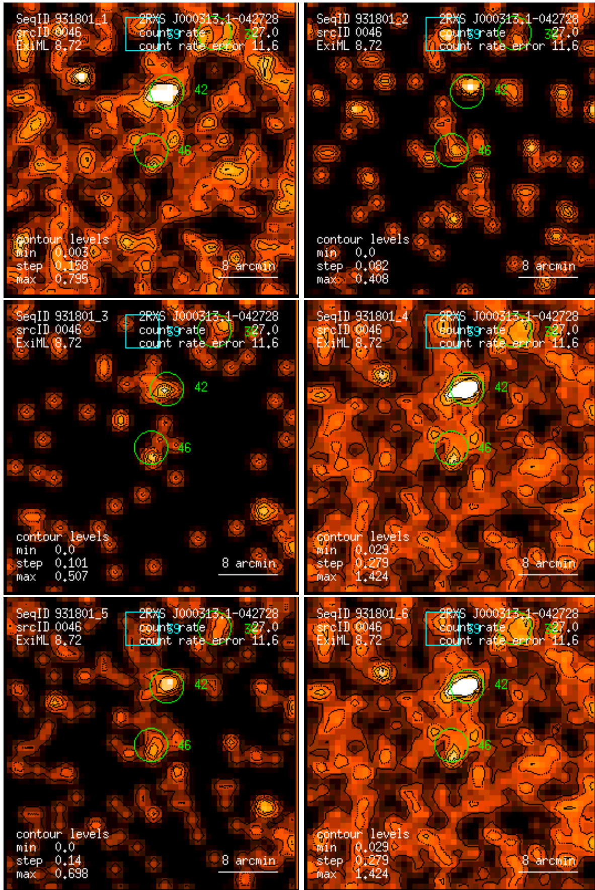
Figure 46: RASS 931801: detection 0046: band rate images, Gaussian filter: (1) PSPC channels 11 – 41, (2) 52 – 90, (3) 91 – 201, (4) 11 – 235, (5) 52 – 201, (6) 11 – 201. Broad band rates in counts/ks. Band rate contour levels in counts/ks/arcmin 2 .
