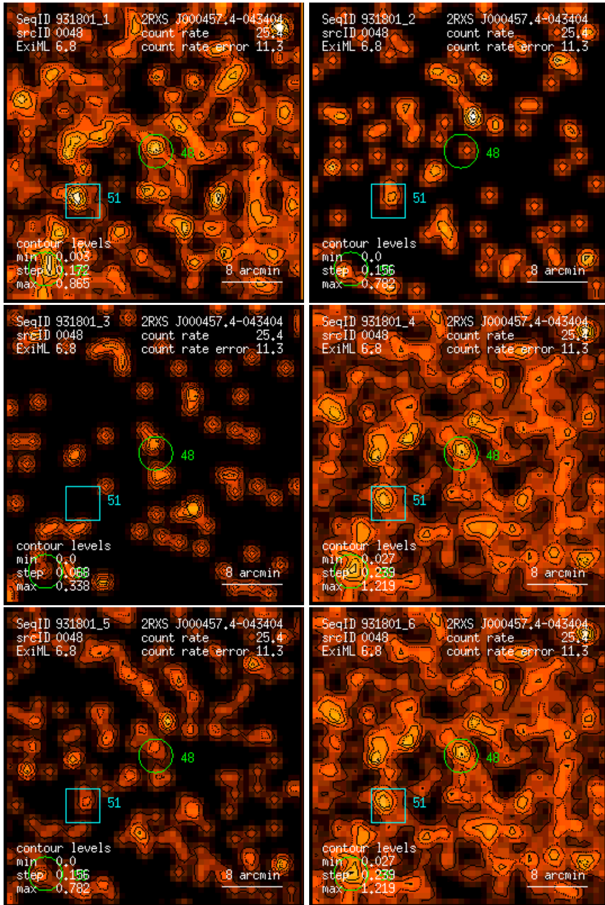
Figure 48: RASS 931801: detection 0048: band rate images, Gaussian filter: (1) PSPC channels 11 – 41, (2) 52 – 90, (3) 91 – 201, (4) 11 – 235, (5) 52 – 201, (6) 11 – 201. Broad band rates in counts/ks. Band rate contour levels in counts/ks/arcmin 2 .
