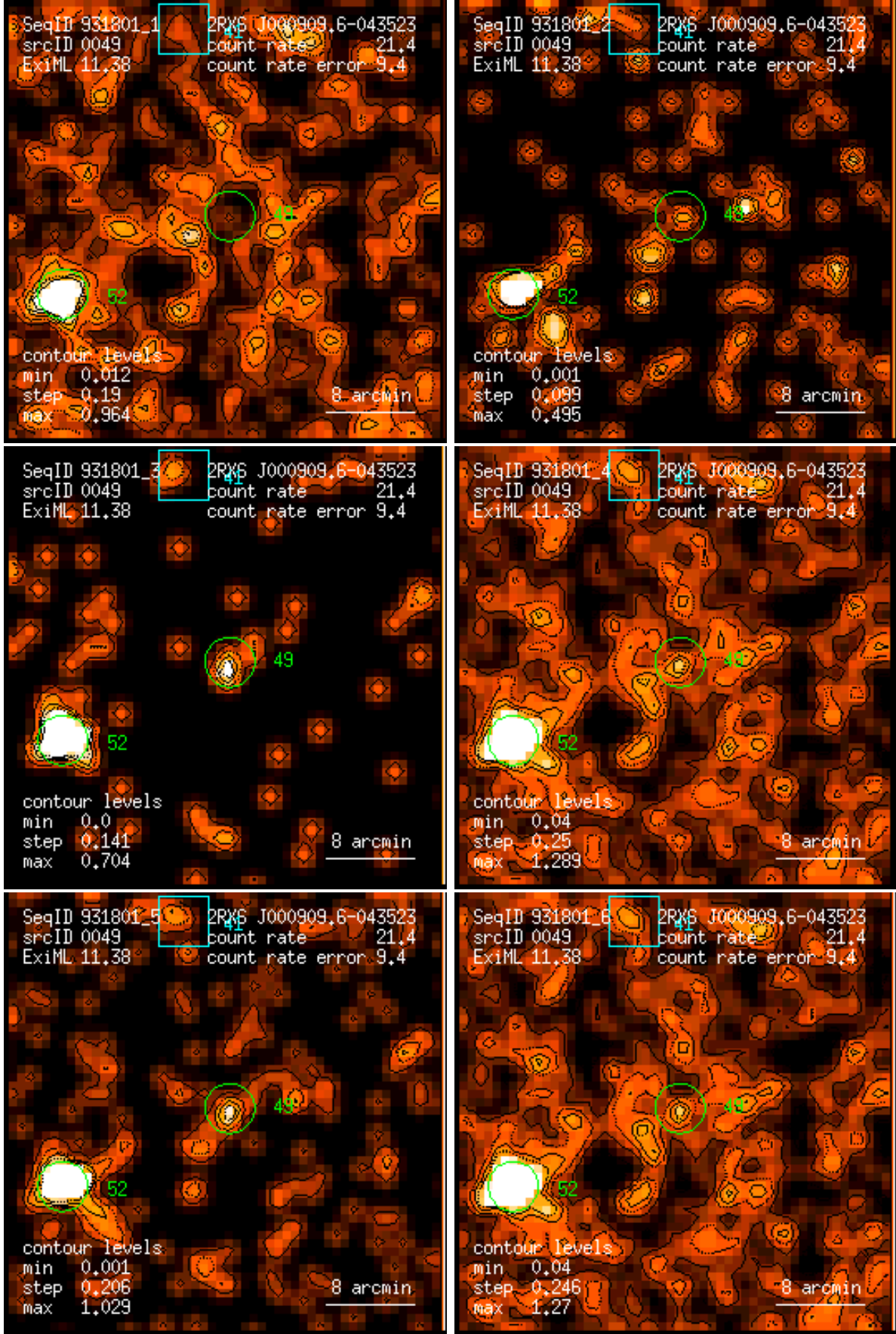
Figure 49: RASS 931801: detection 0049: band rate images, Gaussian filter: (1) PSPC channels 11 – 41, (2) 52 – 90, (3) 91 – 201, (4) 11 – 235, (5) 52 – 201, (6) 11 – 201. Broad band rates in counts/ks. Band rate contour levels in counts/ks/arcmin 2 .
