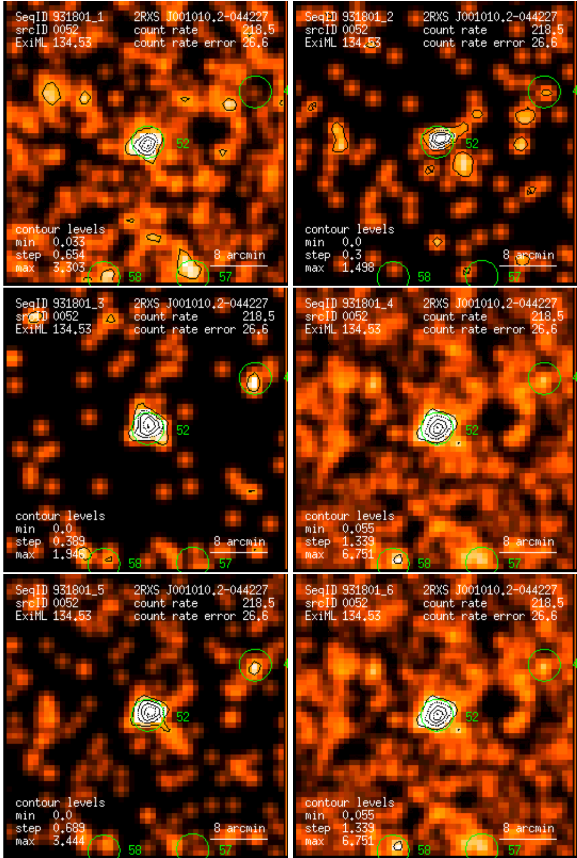
Figure 52: RASS 931801: detection 0052: band rate images, Gaussian filter: (1) PSPC channels 11 – 41, (2) 52 – 90, (3) 91 – 201, (4) 11 – 235, (5) 52 – 201, (6) 11 – 201. Broad band rates in counts/ks. Band rate contour levels in counts/ks/arcmin 2 .
