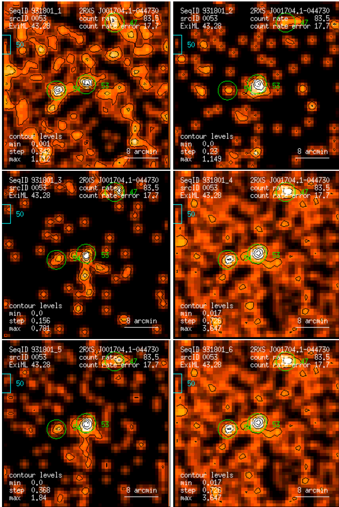
Figure 53: RASS 931801: detection 0053: band rate images, Gaussian filter: (1) PSPC channels 11 – 41, (2) 52 – 90, (3) 91 – 201, (4) 11 – 235, (5) 52 – 201, (6) 11 – 201. Broad band rates in counts/ks. Band rate contour levels in counts/ks/arcmin 2 .
