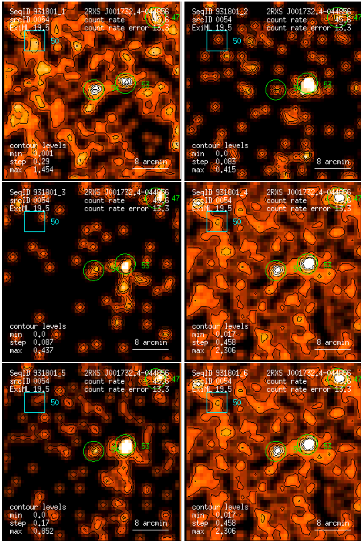
Figure 54: RASS 931801: detection 0054: band rate images, Gaussian filter: (1) PSPC channels 11 – 41, (2) 52 – 90, (3) 91 – 201, (4) 11 – 235, (5) 52 – 201, (6) 11 – 201. Broad band rates in counts/ks. Band rate contour levels in counts/ks/arcmin 2 .
