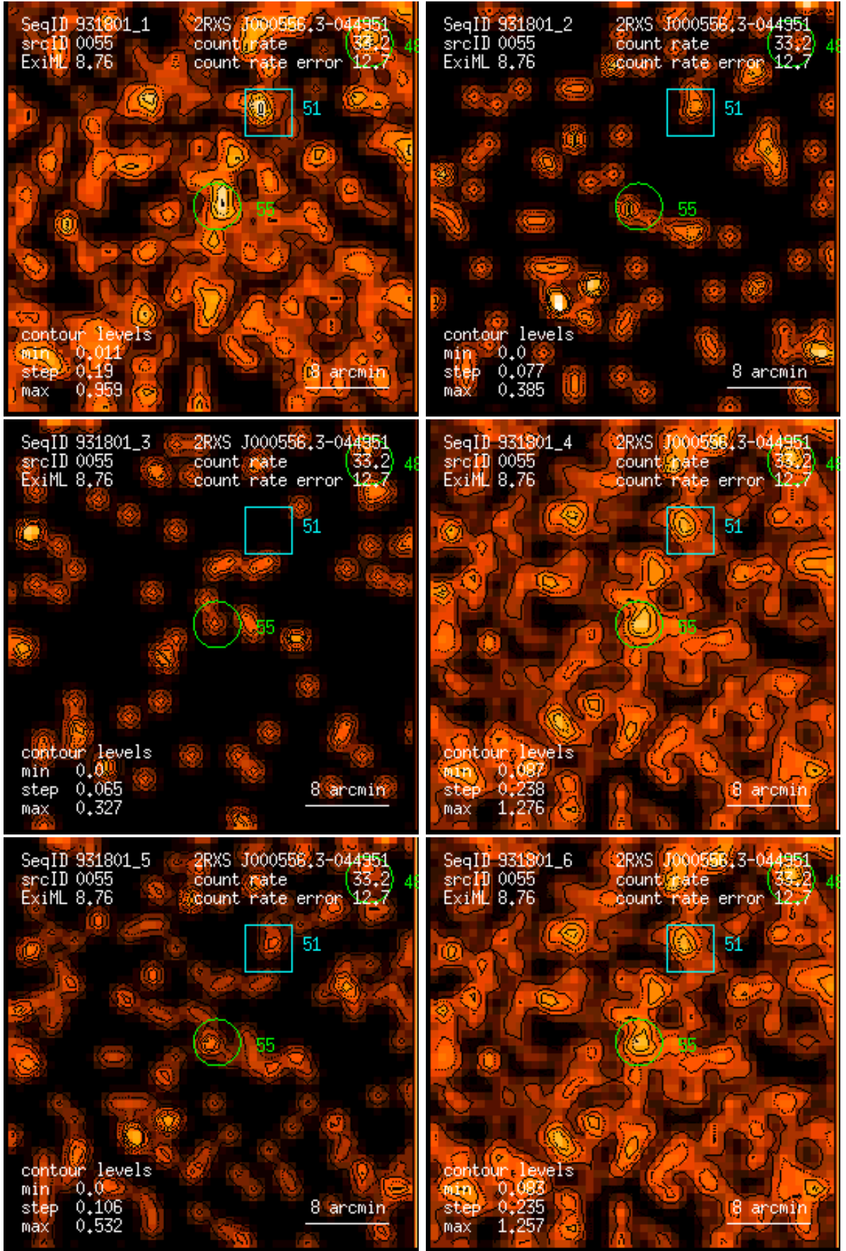
Figure 55: RASS 931801: detection 0055: band rate images, Gaussian filter: (1) PSPC channels 11 – 41, (2) 52 – 90, (3) 91 – 201, (4) 11 – 235, (5) 52 – 201, (6) 11 – 201. Broad band rates in counts/ks. Band rate contour levels in counts/ks/arcmin 2 .
