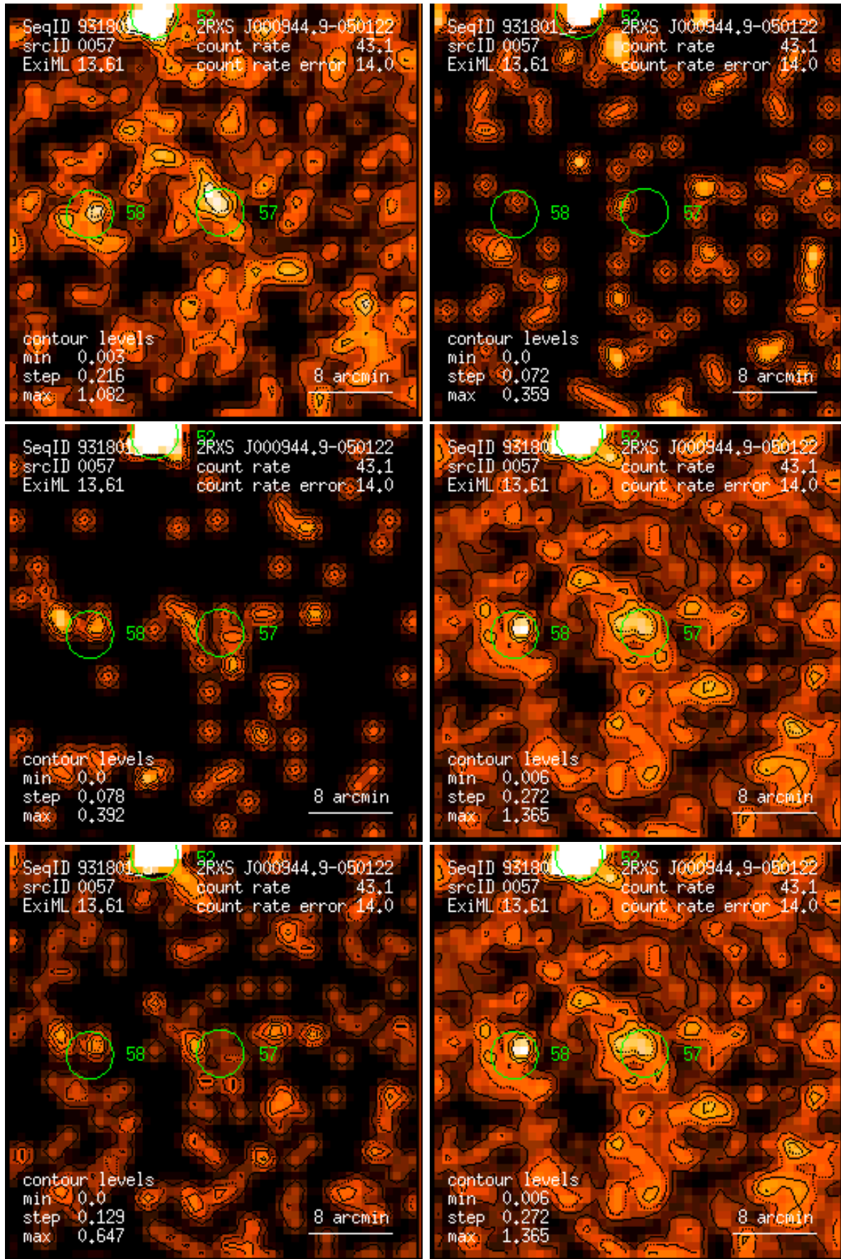
Figure 57: RASS 931801: detection 0057: band rate images, Gaussian filter: (1) PSPC channels 11 – 41, (2) 52 – 90, (3) 91 – 201, (4) 11 – 235, (5) 52 – 201, (6) 11 – 201. Broad band rates in counts/ks. Band rate contour levels in counts/ks/arcmin 2 .
