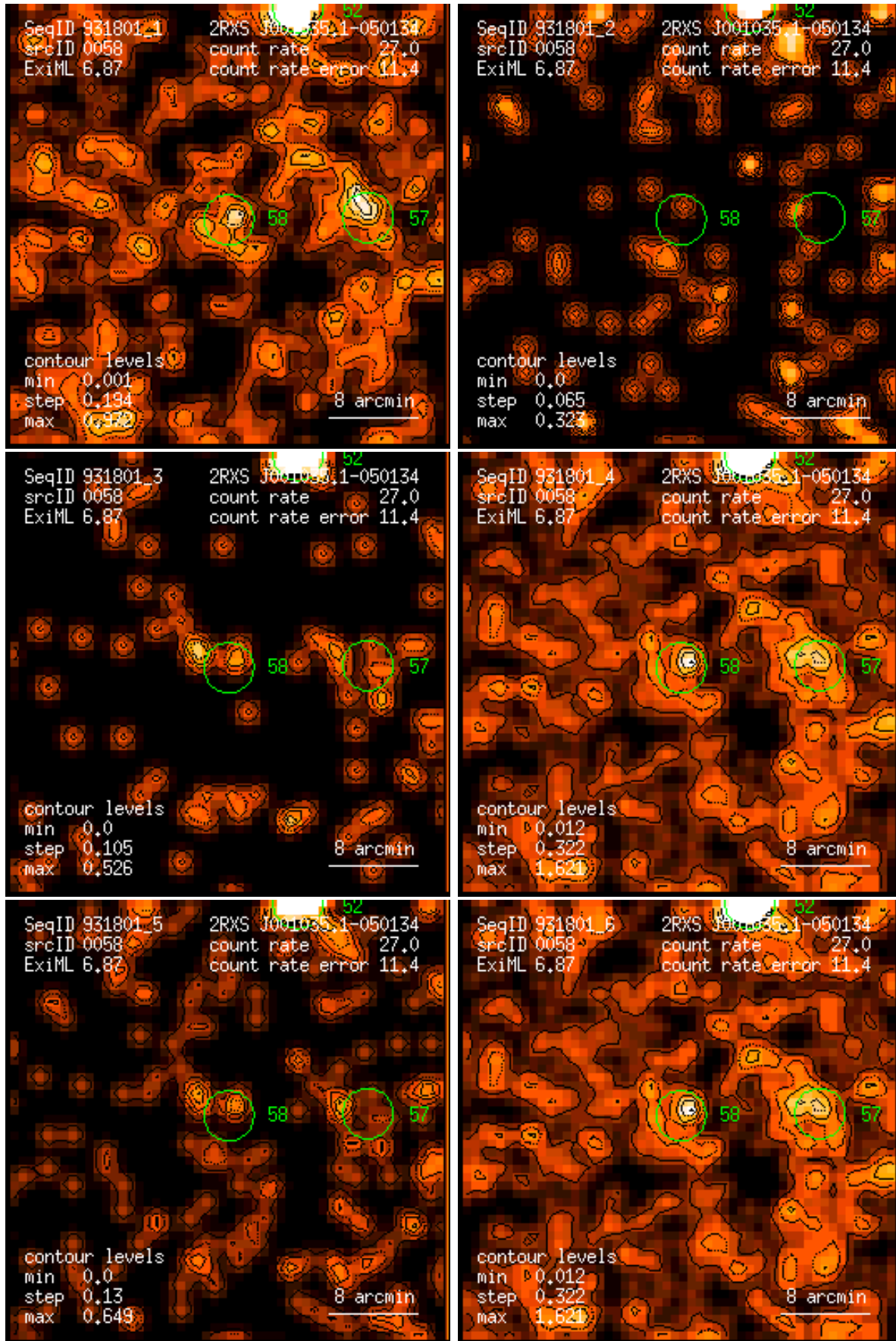
Figure 58: RASS 931801: detection 0058: band rate images, Gaussian filter: (1) PSPC channels 11 – 41, (2) 52 – 90, (3) 91 – 201, (4) 11 – 235, (5) 52 – 201, (6) 11 – 201. Broad band rates in counts/ks. Band rate contour levels in counts/ks/arcmin 2 .
