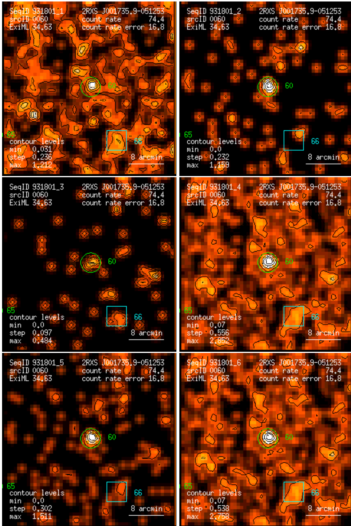
Figure 60: RASS 931801: detection 0060: band rate images, Gaussian filter: (1) PSPC channels 11 – 41, (2) 52 – 90, (3) 91 – 201, (4) 11 – 235, (5) 52 – 201, (6) 11 – 201. Broad band rates in counts/ks. Band rate contour levels in counts/ks/arcmin 2 .
