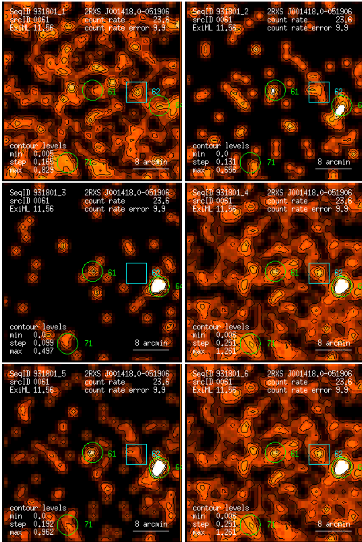
Figure 61: RASS 931801: detection 0061: band rate images, Gaussian filter: (1) PSPC channels 11 – 41, (2) 52 – 90, (3) 91 – 201, (4) 11 – 235, (5) 52 – 201, (6) 11 – 201. Broad band rates in counts/ks. Band rate contour levels in counts/ks/arcmin 2 .
