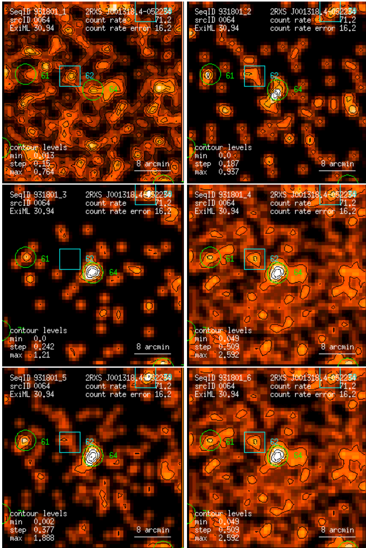
Figure 64: RASS 931801: detection 0064: band rate images, Gaussian filter: (1) PSPC channels 11 – 41, (2) 52 – 90, (3) 91 – 201, (4) 11 – 235, (5) 52 – 201, (6) 11 – 201. Broad band rates in counts/ks. Band rate contour levels in counts/ks/arcmin 2 .
