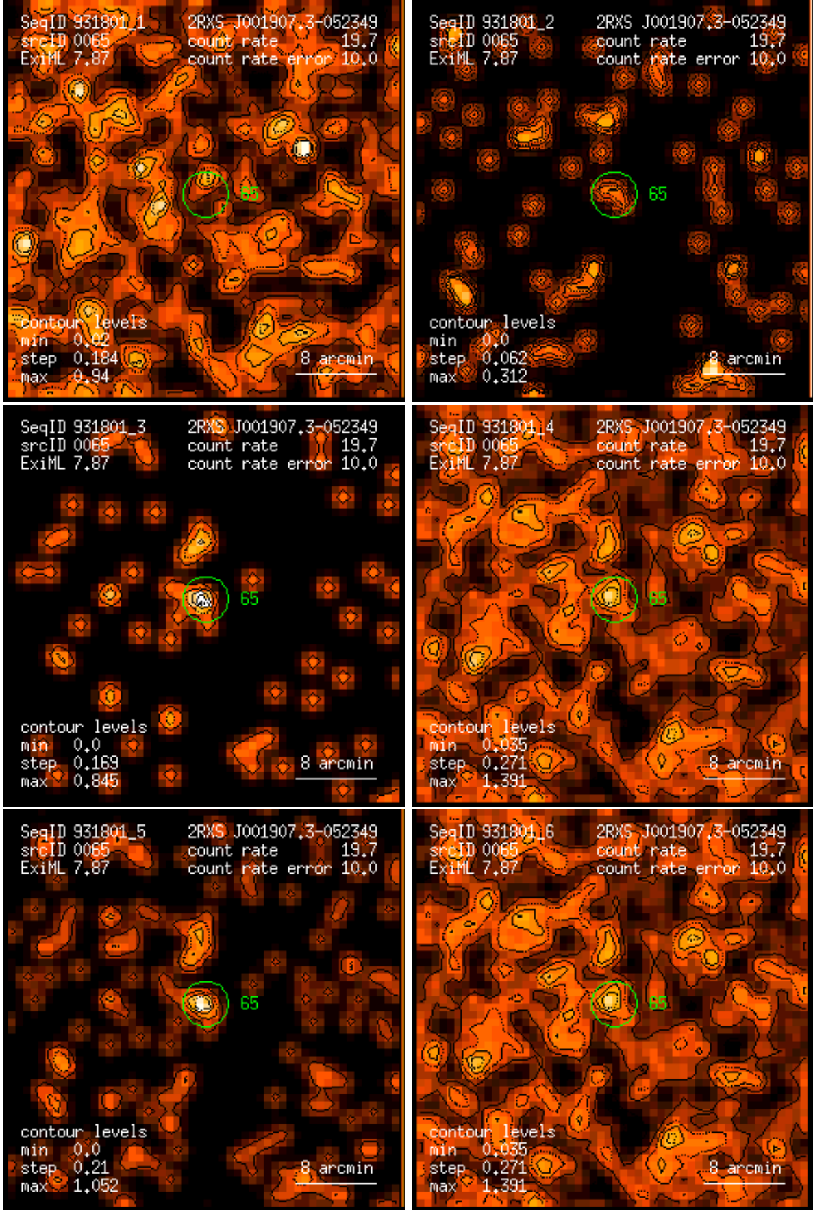
Figure 65: RASS 931801: detection 0065: band rate images, Gaussian filter: (1) PSPC channels 11 – 41, (2) 52 – 90, (3) 91 – 201, (4) 11 – 235, (5) 52 – 201, (6) 11 – 201. Broad band rates in counts/ks. Band rate contour levels in counts/ks/arcmin 2 .
