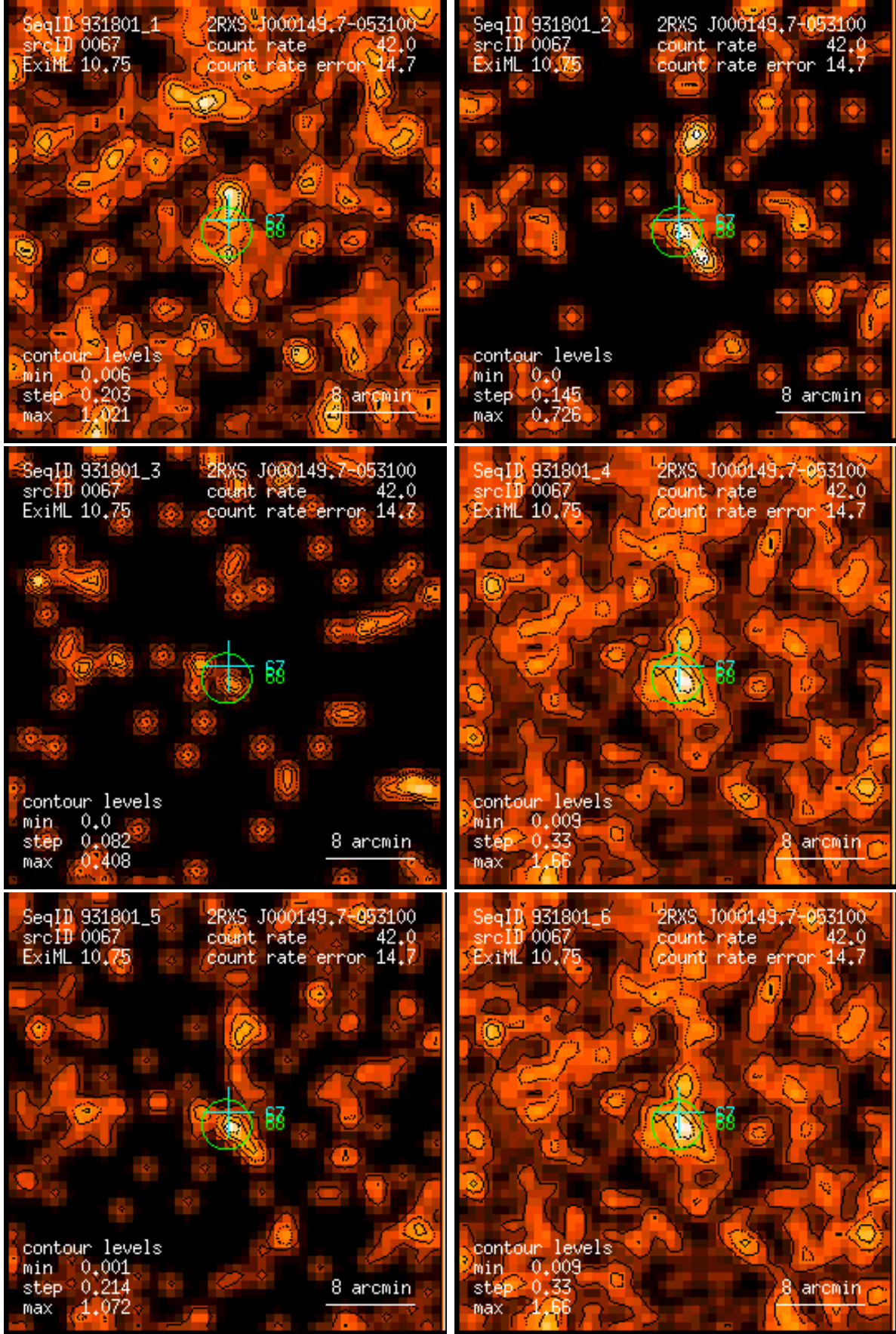
Figure 67: RASS 931801: detection 0067: band rate images, Gaussian filter: (1) PSPC channels 11 – 41, (2) 52 – 90, (3) 91 – 201, (4) 11 – 235, (5) 52 – 201, (6) 11 – 201. Broad band rates in counts/ks. Band rate contour levels in counts/ks/arcmin 2 .
