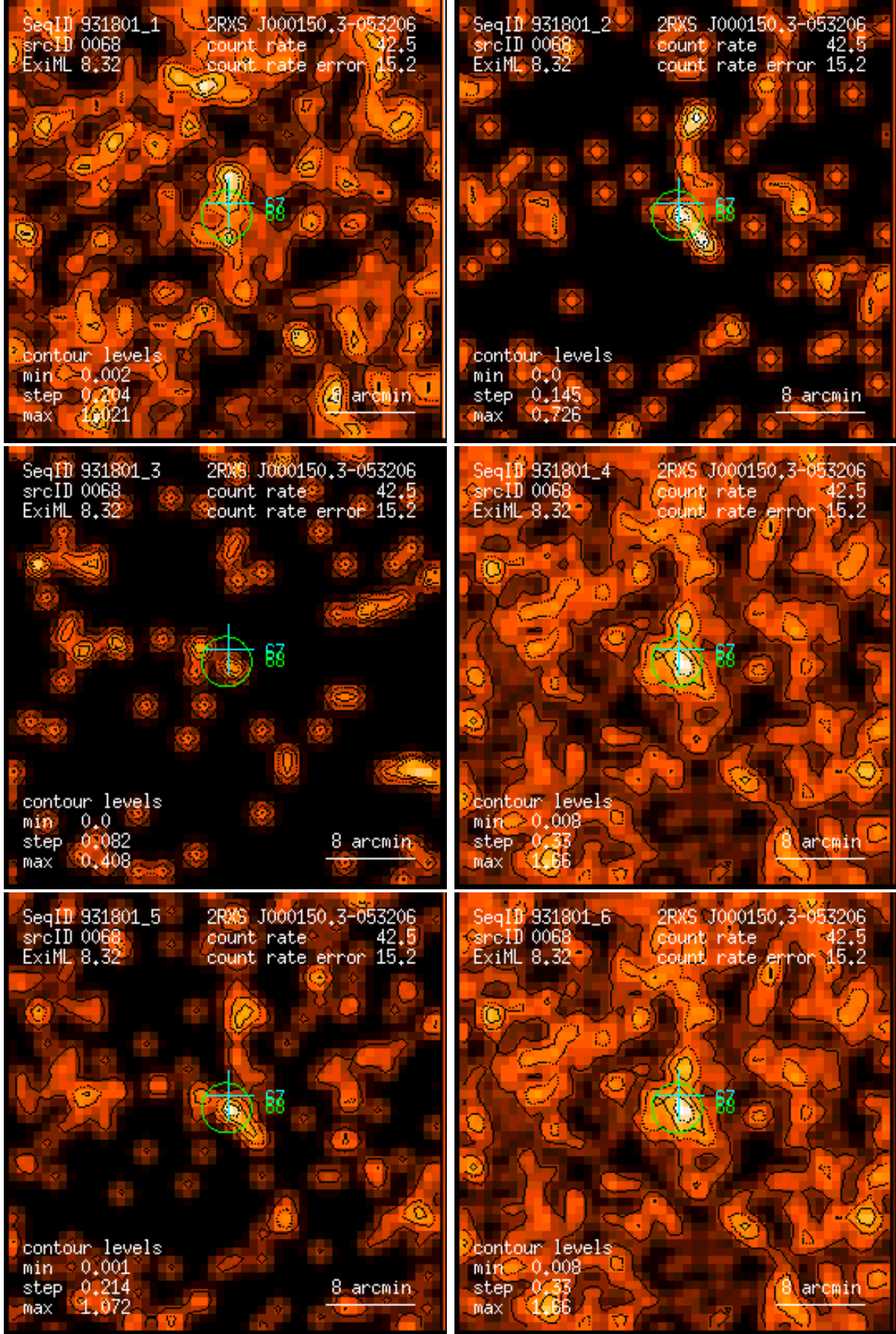
Figure 68: RASS 931801: detection 0068: band rate images, Gaussian filter: (1) PSPC channels 11 – 41, (2) 52 – 90, (3) 91 – 201, (4) 11 – 235, (5) 52 – 201, (6) 11 – 201. Broad band rates in counts/ks. Band rate contour levels in counts/ks/arcmin 2 .
